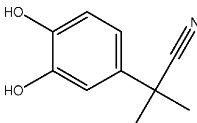
2-(3,4-dihydroxyphenyl)-2-methylpropanenitrile Compound 10
