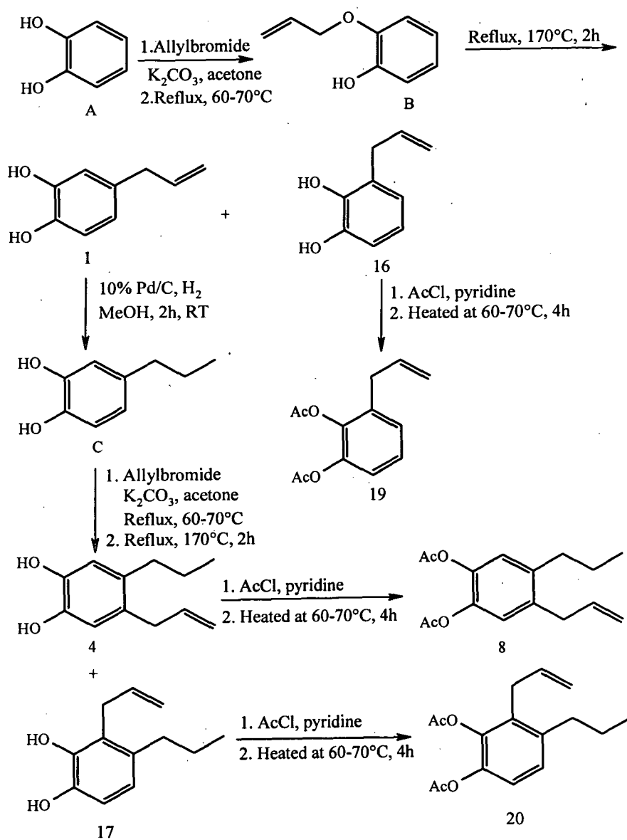
Scheme 1
