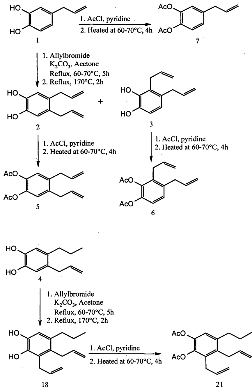
Scheme 2
