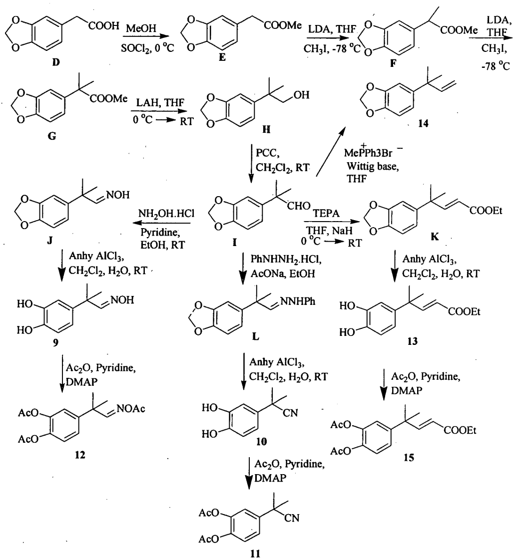
Scheme 3
