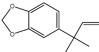
5-(2-methylbut-3-en-2-yl)benzo[d][1,3]dioxole Compound 14
