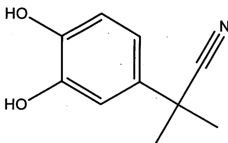
2-(3,4-dihydroxyphenyl)-2-methylpropanenitrile Compound 10
