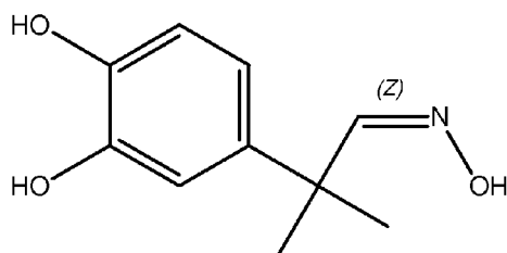
2-(3,4-Dihydroxyphenyl)-2-methylpropanaloxim Verbindung 9
