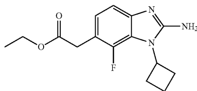
ethyl 2-(2-amino-7-fluoro-1-(4-fluorophenyl)-1H-benzo[d]imidazol-6-yl)acetate
