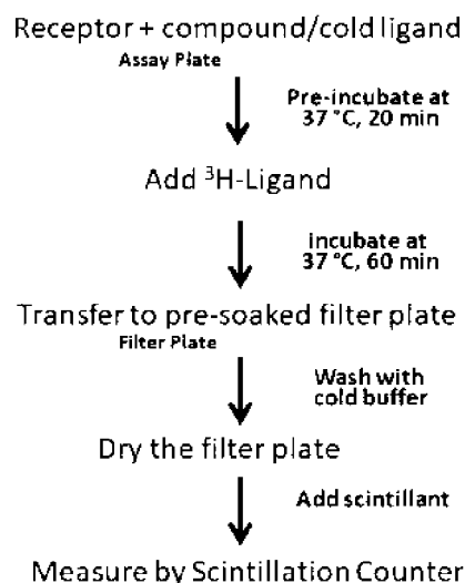
Scheme 8 Schematic representation of the radioligand binding assay for CB1 and CB2
