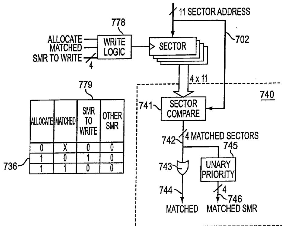
Sector match logic
