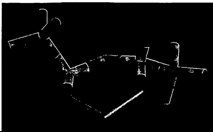
Figure 3: The structure of Zn(NH 2 ) 2 .
