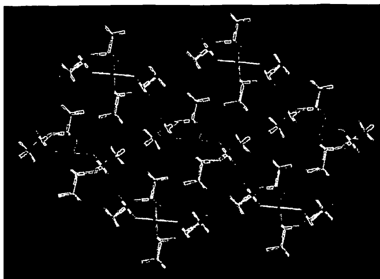
Figure 6, The structure of \text{Zn}(\text{NTf}_2)_2 .
