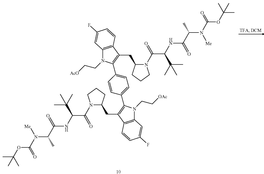
Scheme V
