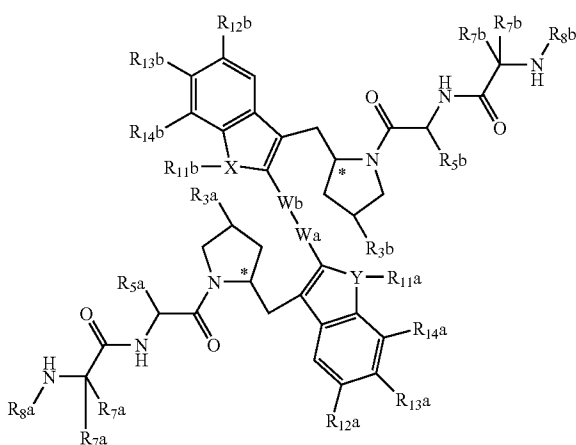
Example 2
