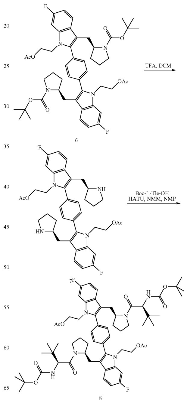
Scheme III
