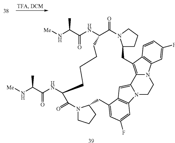
Scheme XIX
