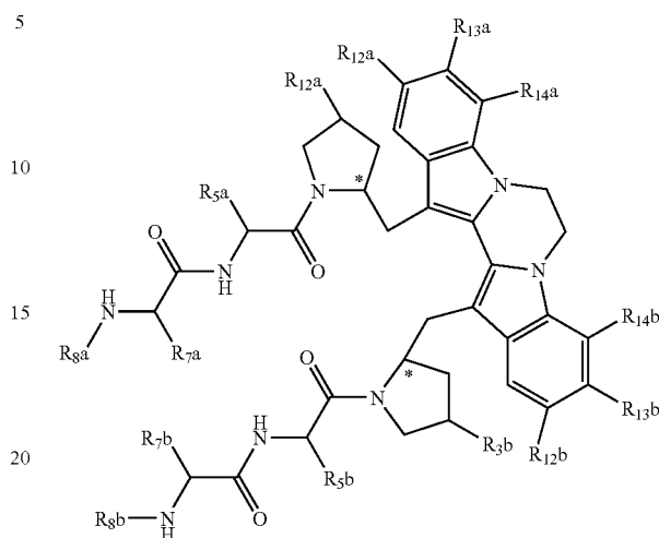
Example 4
