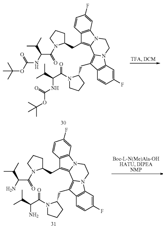
Scheme XII
