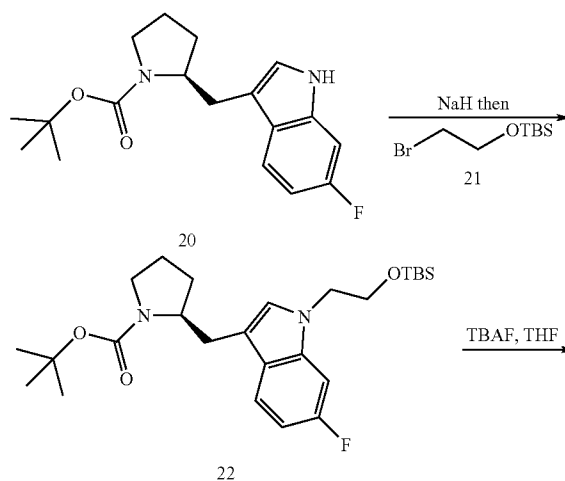
Scheme VIII
