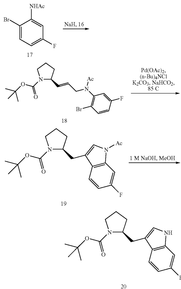
Scheme VII
