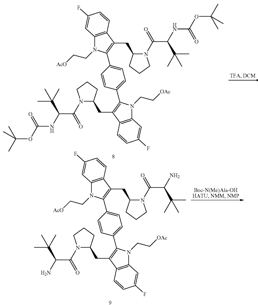
Scheme IV
