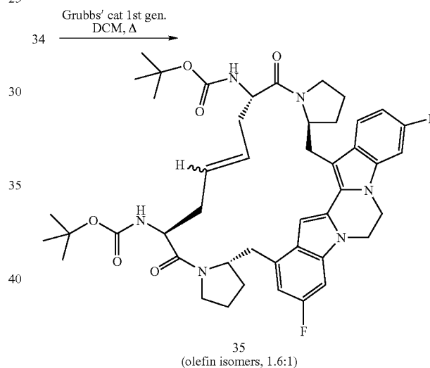
Scheme XV
