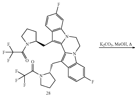
Scheme XI
