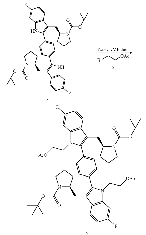
Scheme II
