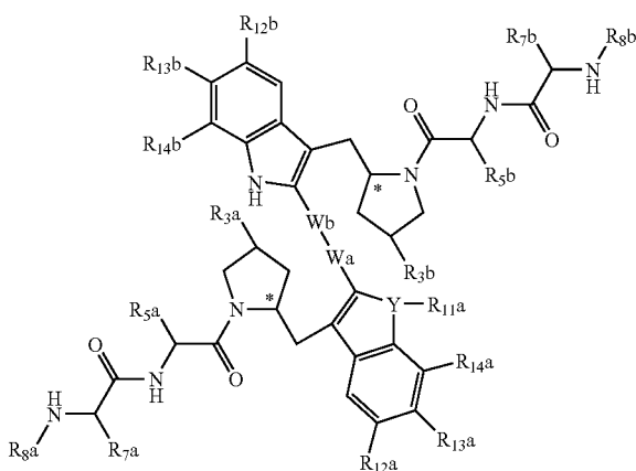
Example 3
