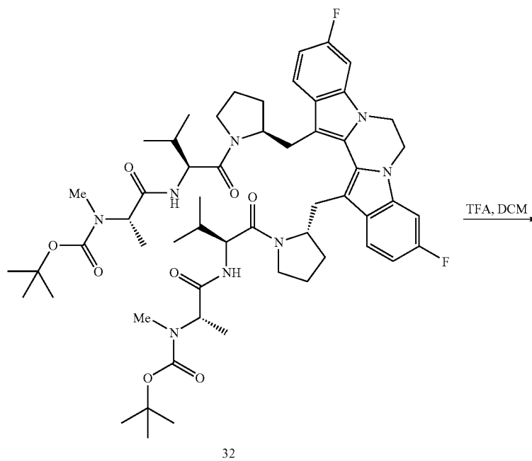
Scheme XIII
