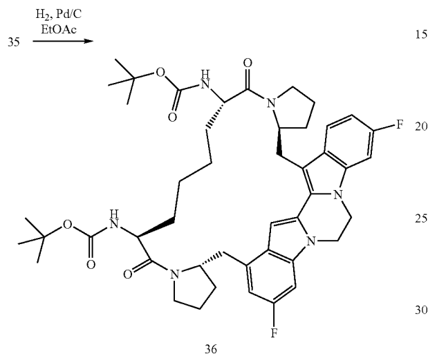
Scheme XVII
