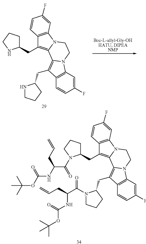
Scheme XIV
