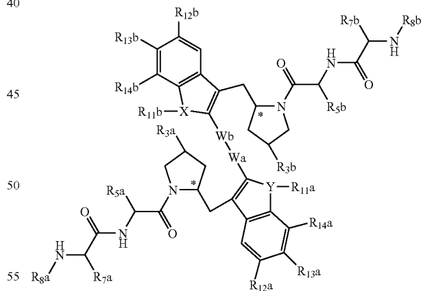
Example 1
