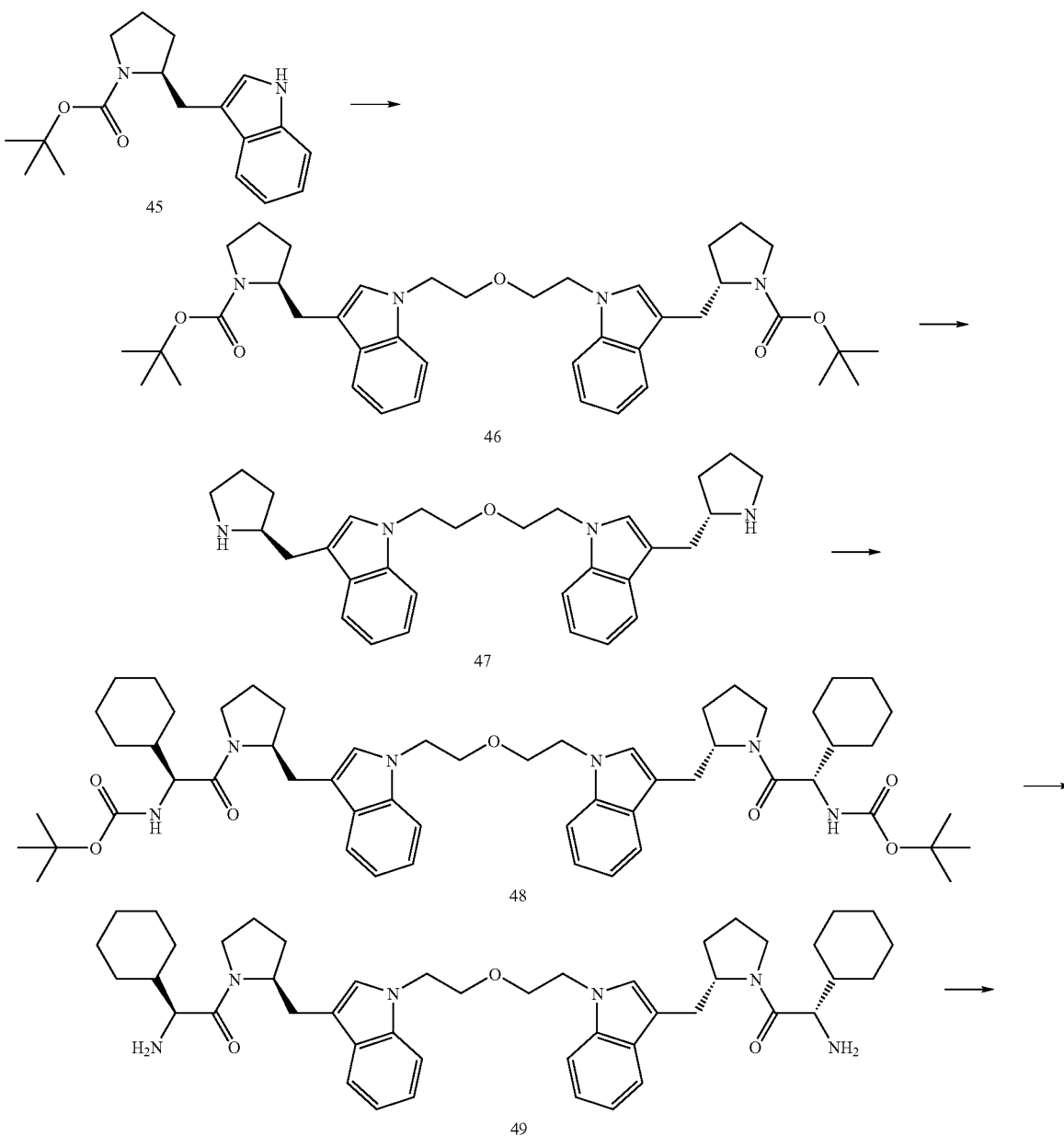
Scheme XXI
