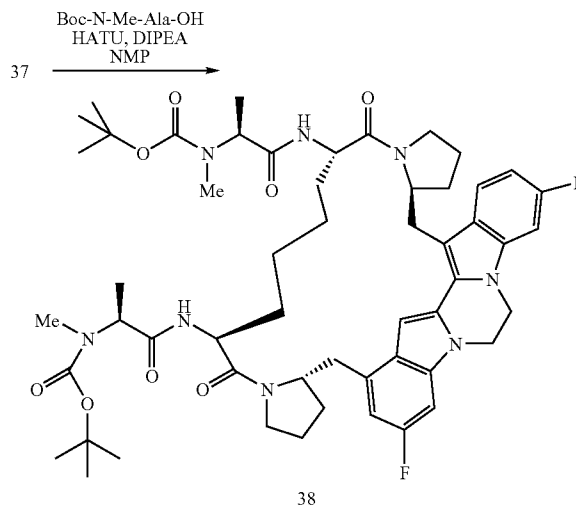
Scheme XVIII
