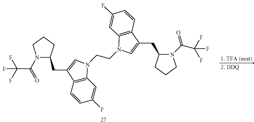
Scheme X
