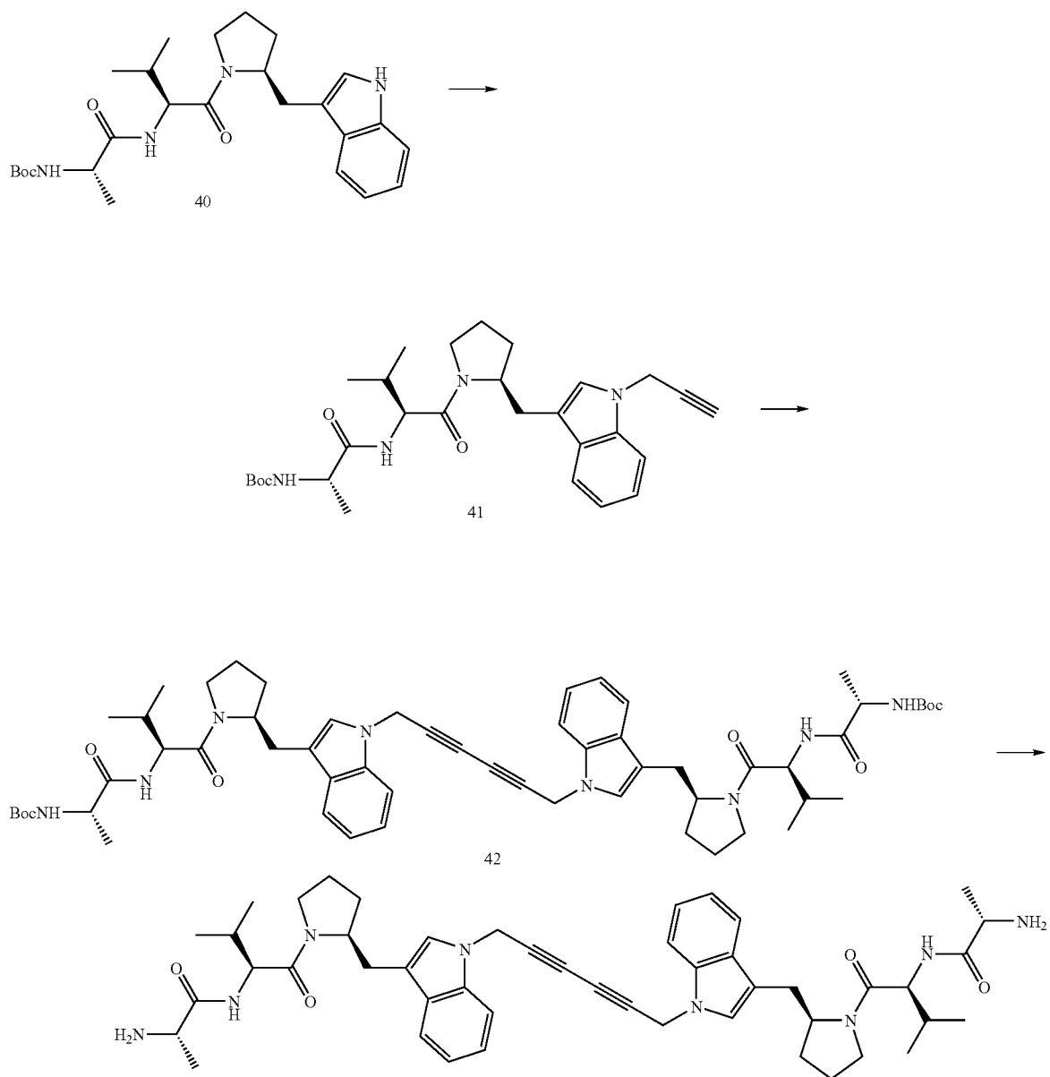
Scheme XX
