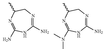
7-ring cyclic biguanides: Formula (IV)
