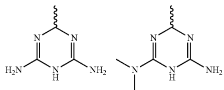
Dihydrotriazines: Formula (III)
