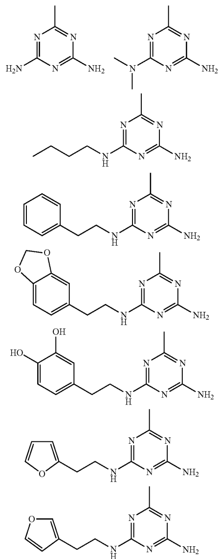
Triazines: Formula (II)
