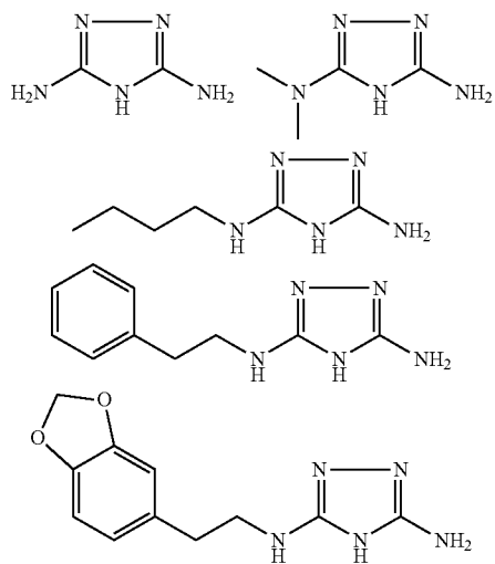
Triazoles: Formula (IA)
