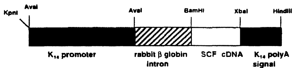
TRANSGENE 1
