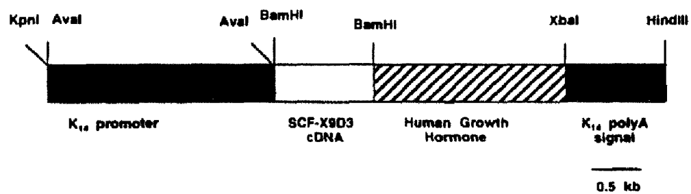
TRANSGENE 2
