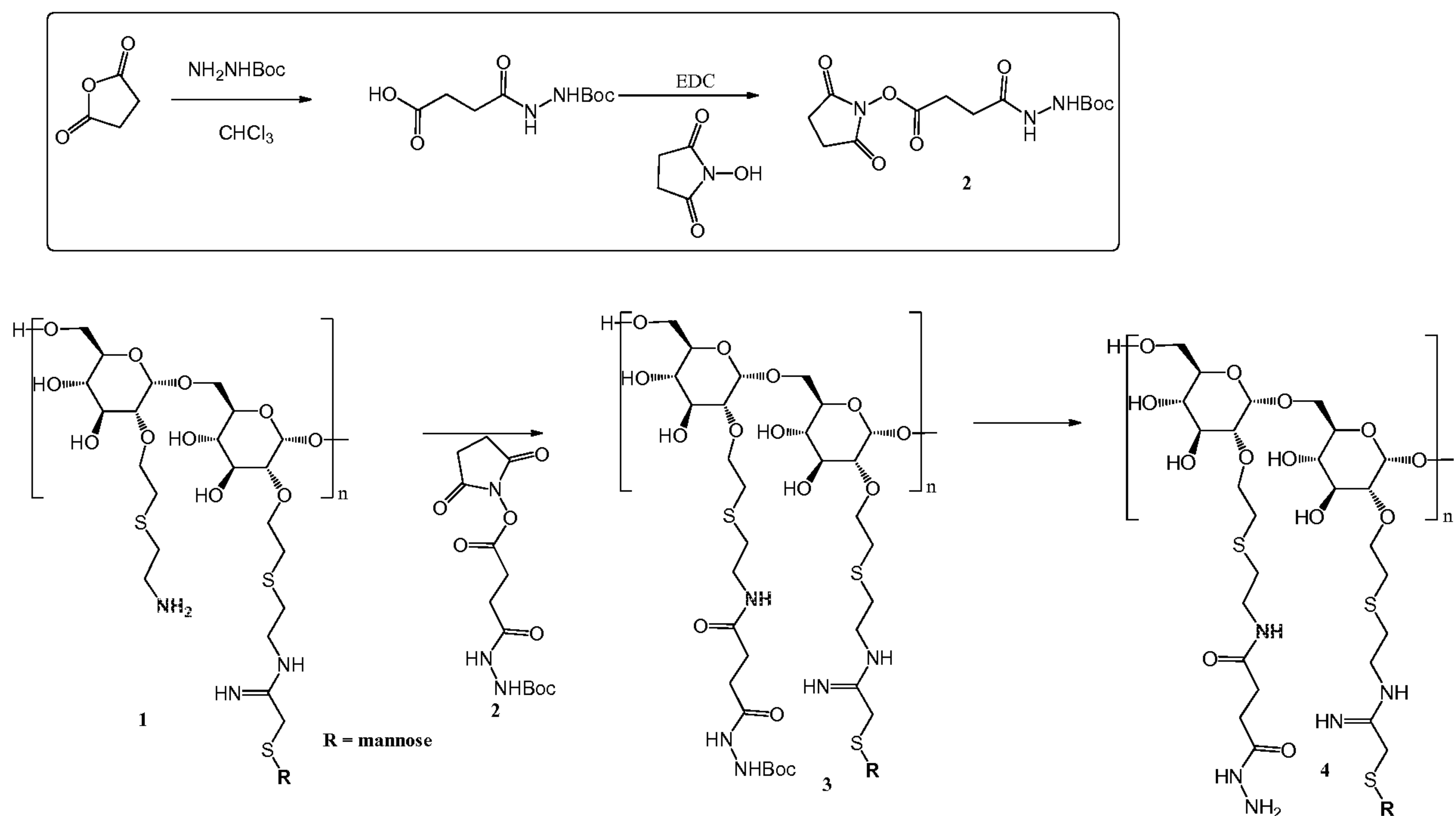
Scheme 1: Synthetic route A for the modification of tilmanocept
