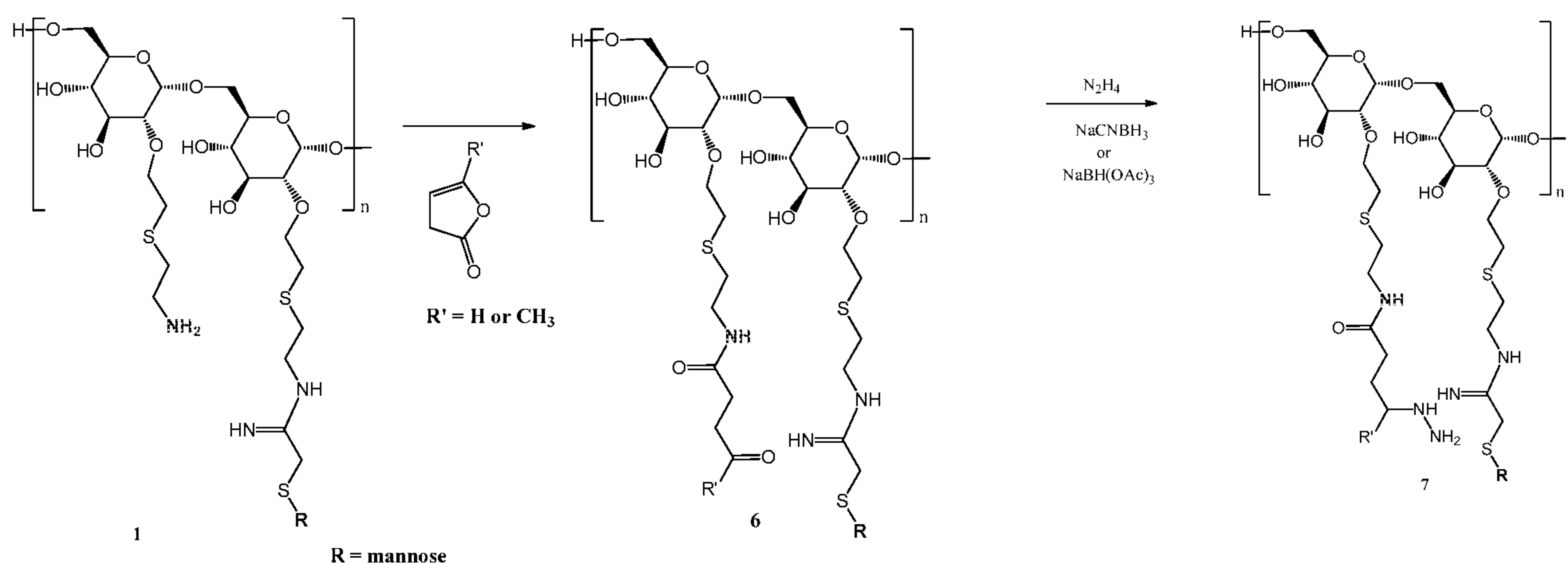
Scheme 2: Synthetic route B for the modification of tilmanocept
