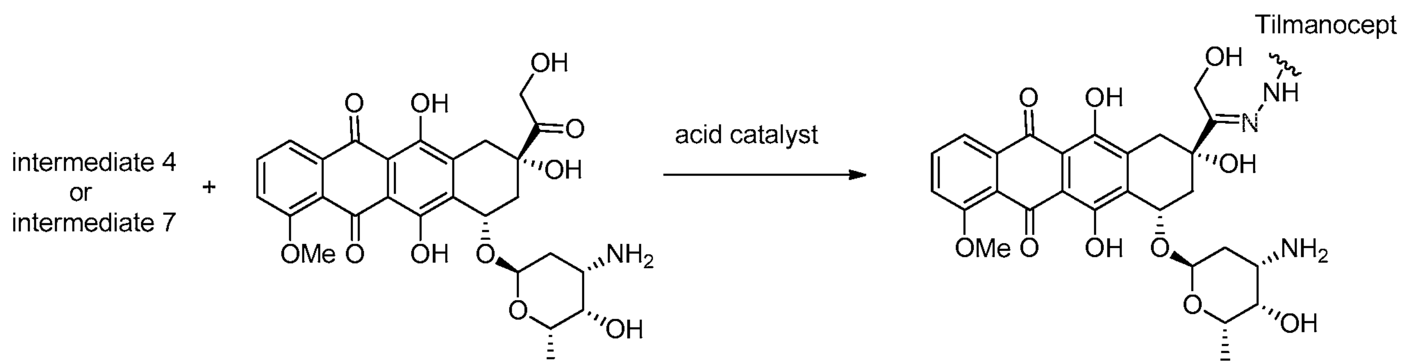
Scheme 3: Conjugation of doxorubicin to tilmanocept derivatives
