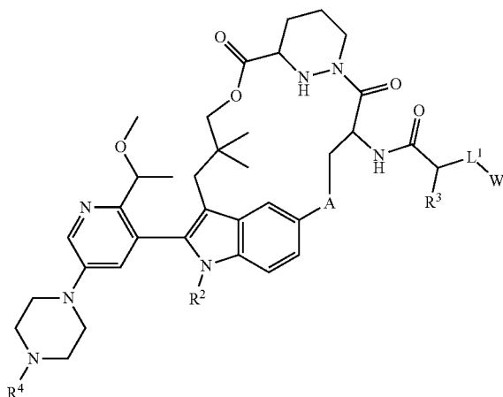
Formula II-3
