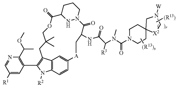
Formula II-5b
