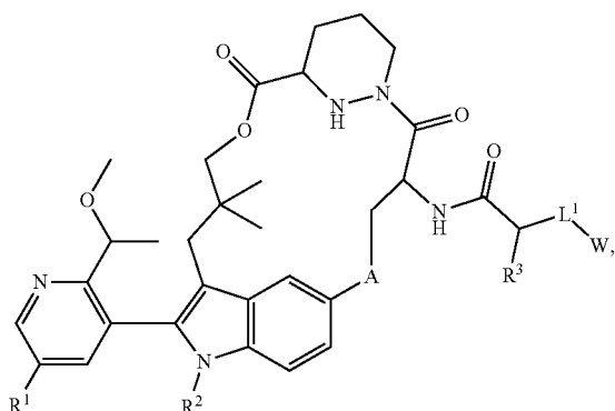
Formula I
