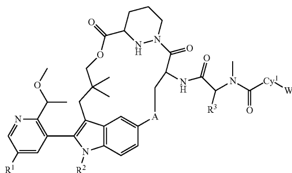
Formula II-5
