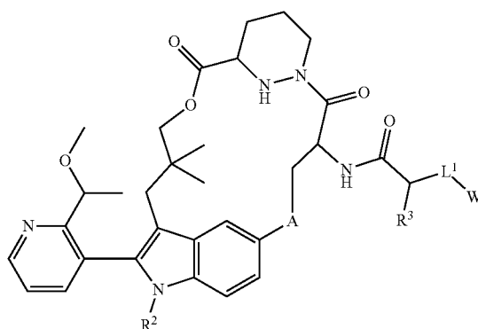
Formula II-1
