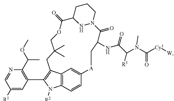
Formula II-5
