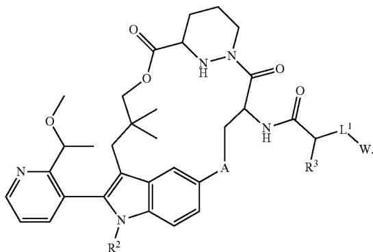
Formula II-1
