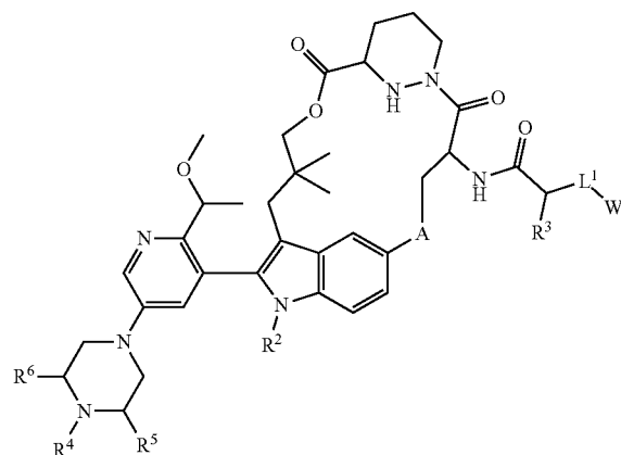
Formula II-2
