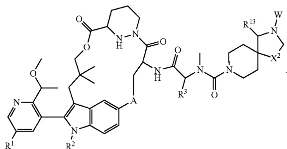
Formula II-5c
