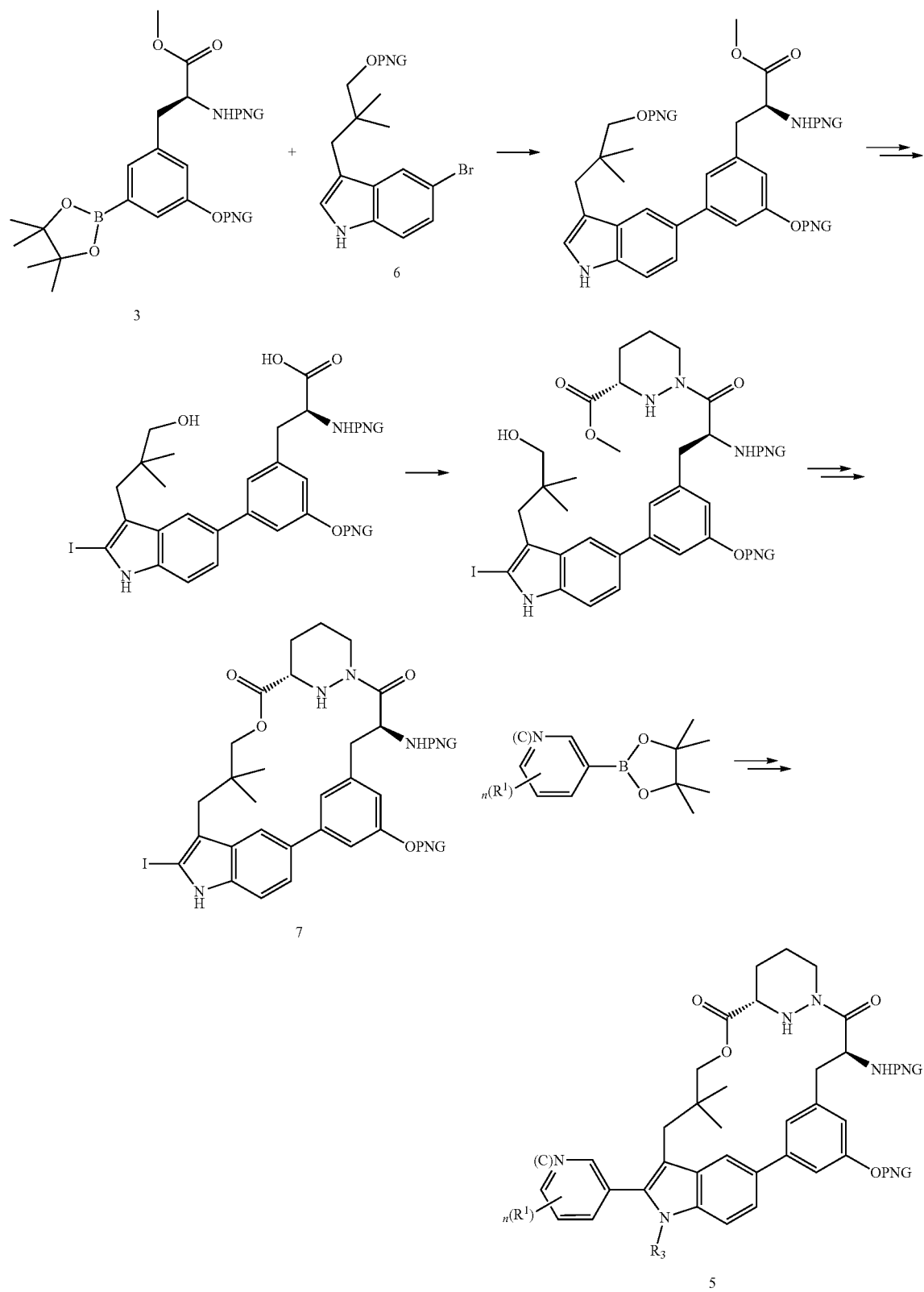
Scheme 2. Alternative general synthesis of macrocyclic esters
