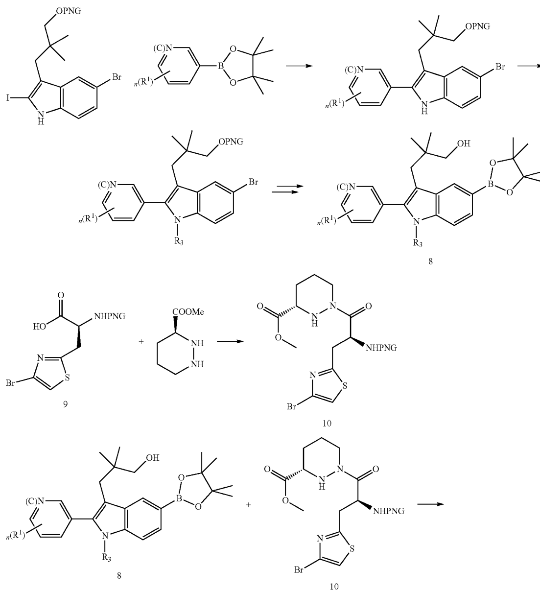
Scheme 3. General synthesis of macrocyclic esters
