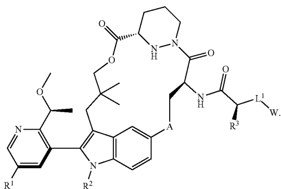
Formula Ia
