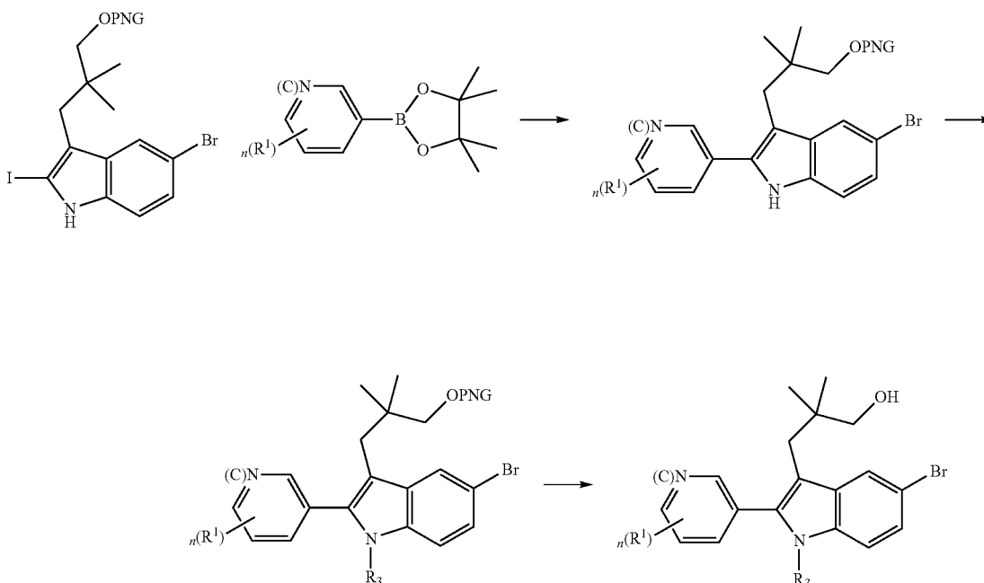
Scheme 1. General synthesis of macrocyclic esters
