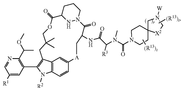
Formula II-5a
