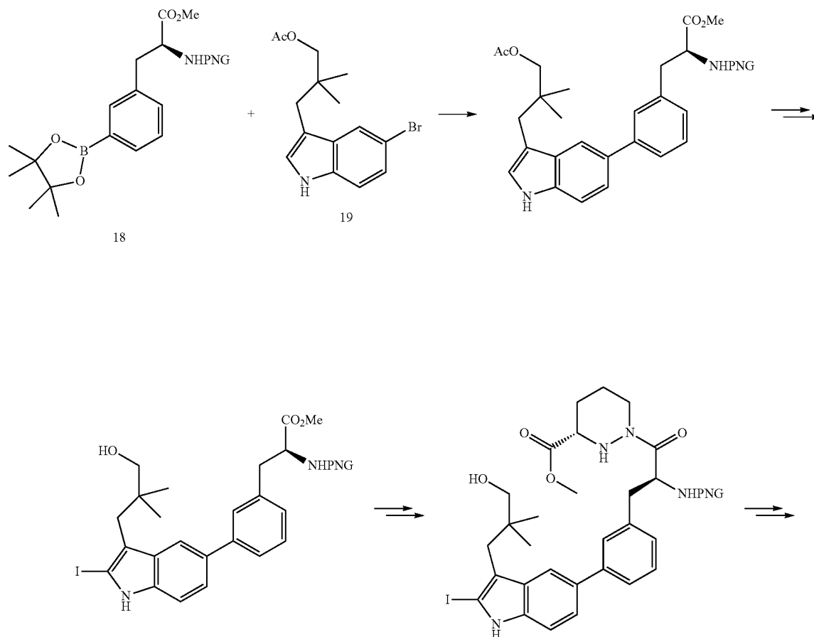
Scheme 5. General synthesis of macrocyclic esters
