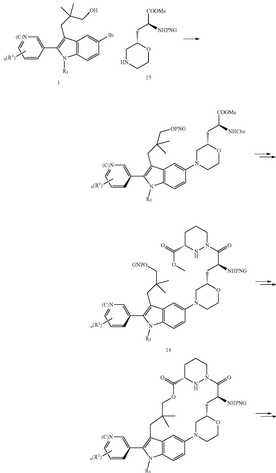
Scheme 4. General synthesis of macrocyclic esters
