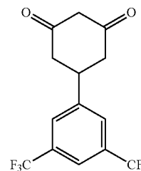
5-(3,5-bis(trifluoromethyl)phenyl)cyclohexane-1,3-dione
