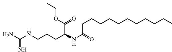
Ethyl N- \alpha -Lauroyl-L-Arginate
