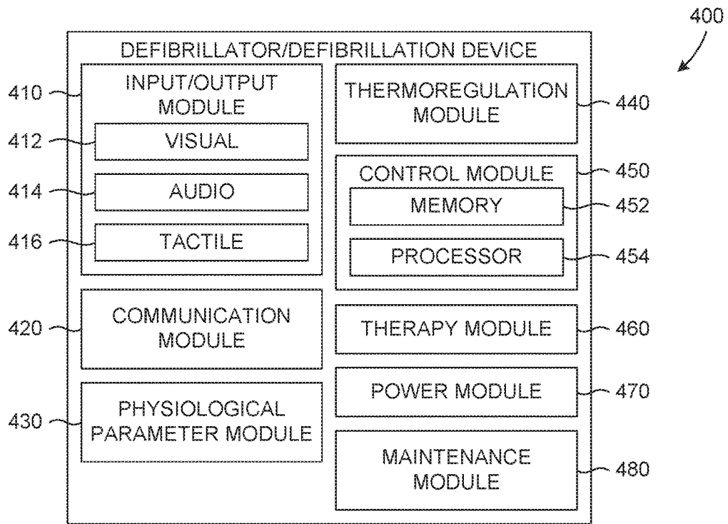
FIG. 4 EXAMPLE DEFIBRILLATION DEVICE
