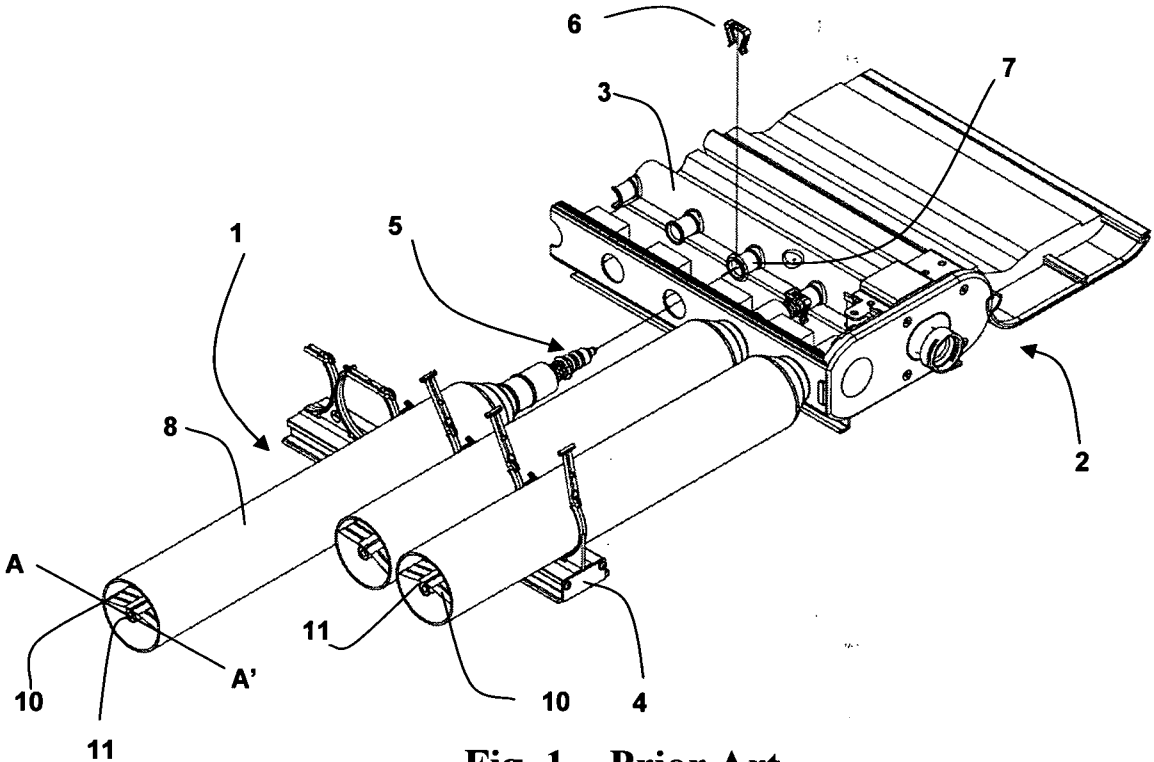
Fig. 1 – Prior Art
