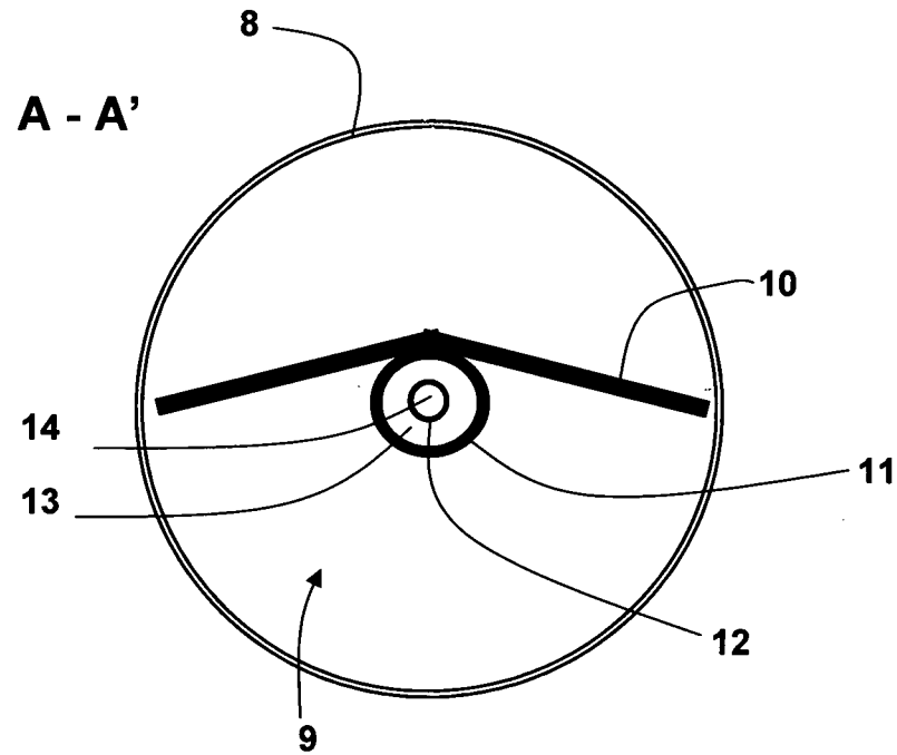
Fig. 3 – Prior Art
