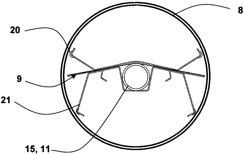
Fig. 7 – Prior Art
