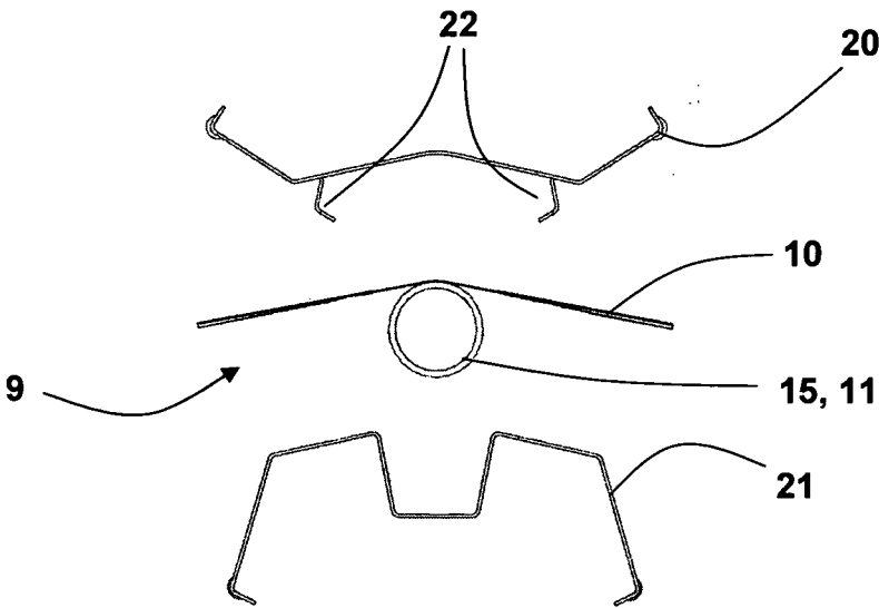
Fig. 5 – Prior Art
