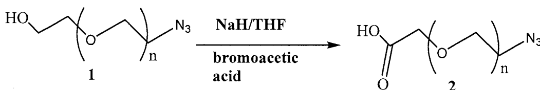
Scheme 1. Synthesis of 2 .
