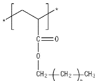
[Chemical Formula 3-1]
