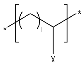
[Chemical Formula 3]
