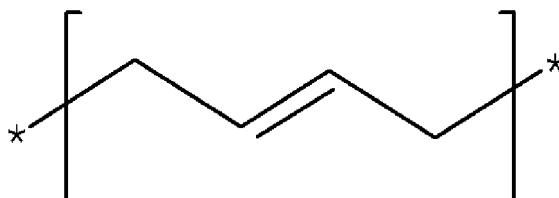
[Chemical Formula 4]
