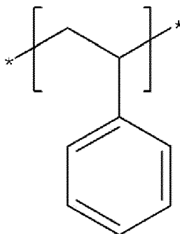
[Chemical Formula 2]
