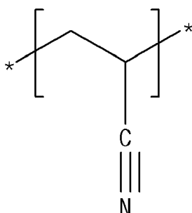
[Chemical Formula 3]
