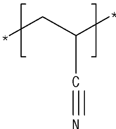
[Chemical Formula 3]
