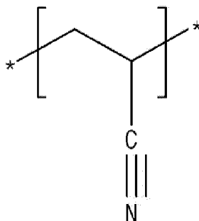
[Chemical Formula 3]
