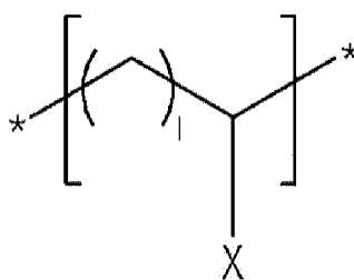
[Chemical Formula 3]
