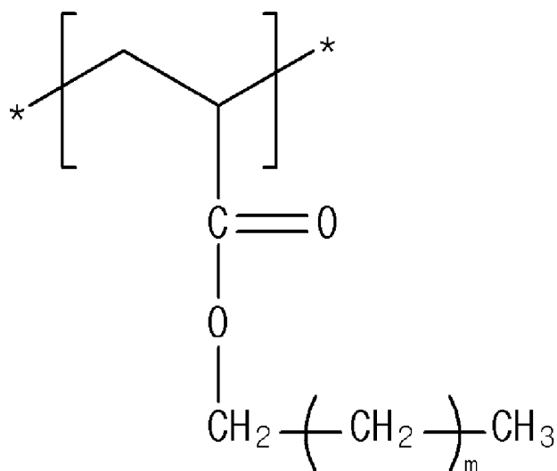
[Chemical Formula 3-1]
