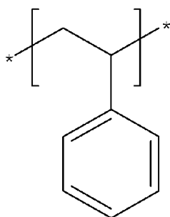
[Chemical Formula 1]
