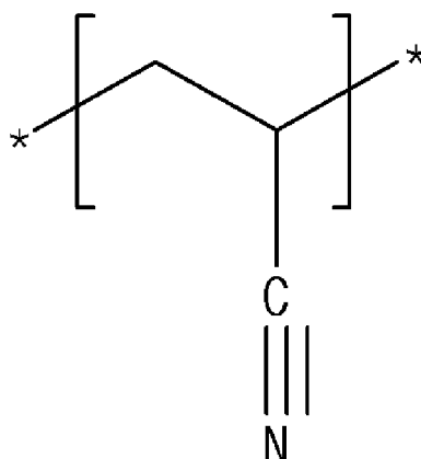
[Chemical Formula 3]
