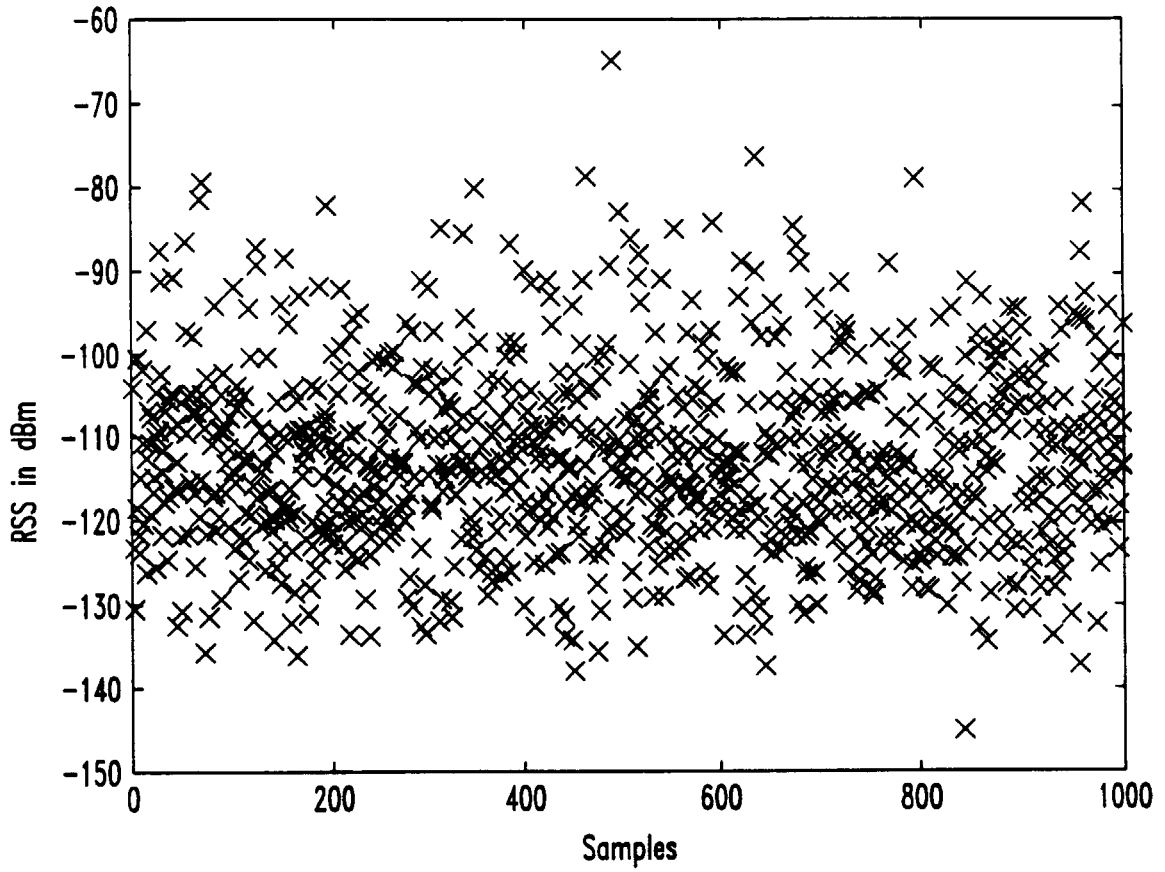
A Typical Received Signal Strength (RSS) Distribution
