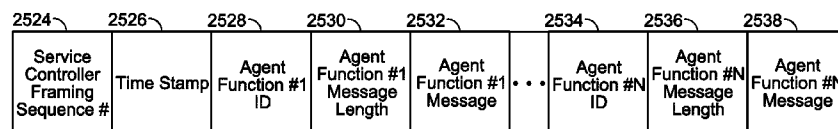
Service Controller Communication Frame 2522
