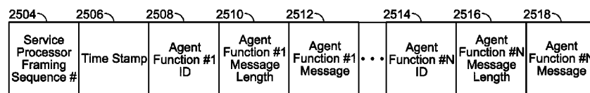
Service Processor Communication Frame 2502
