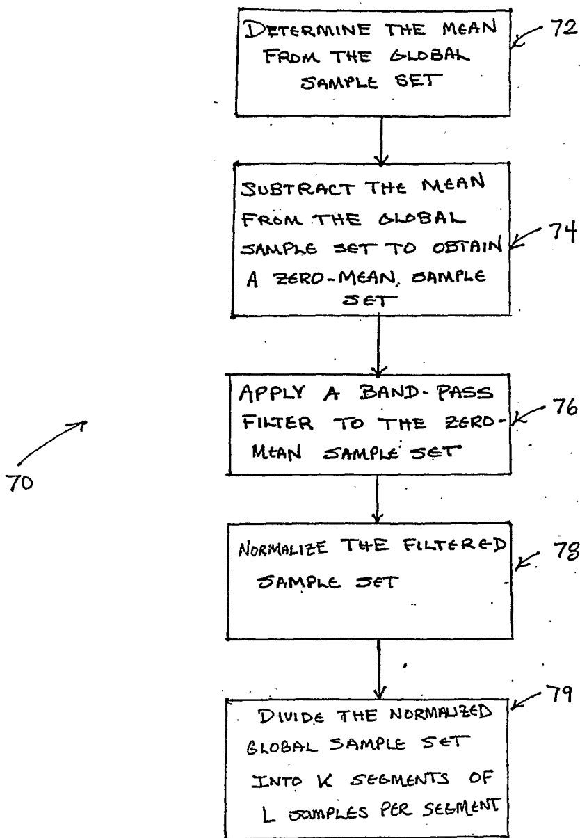
Fig. 13: Signal Preparation
