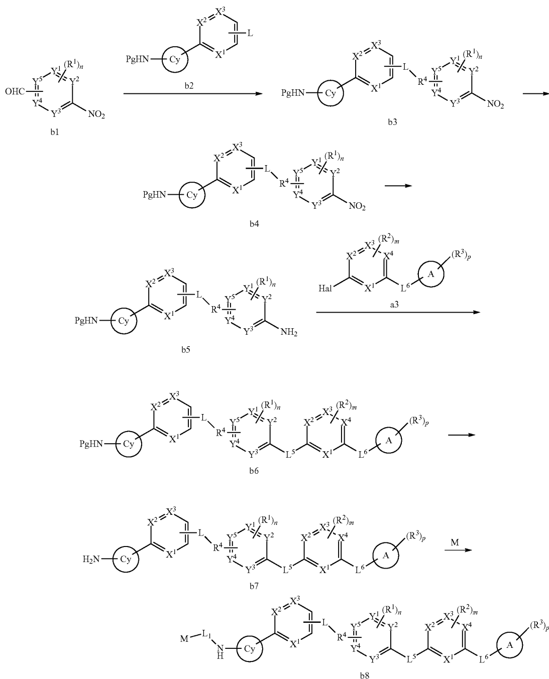
Synthesis Scheme (2):
