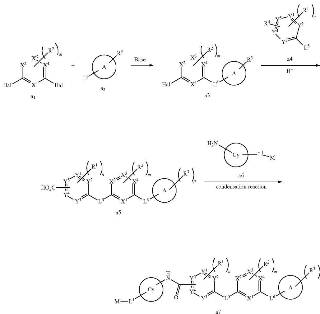
Synthesis Scheme (1):
