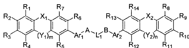
Chemical Formula 1
