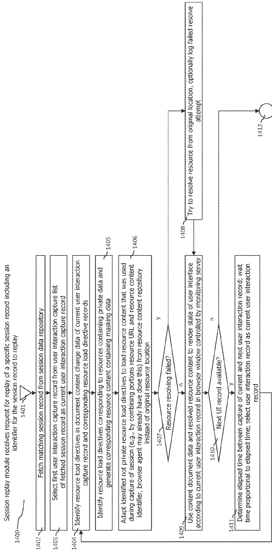
FIG. 14 Replay of Session Recording Data
