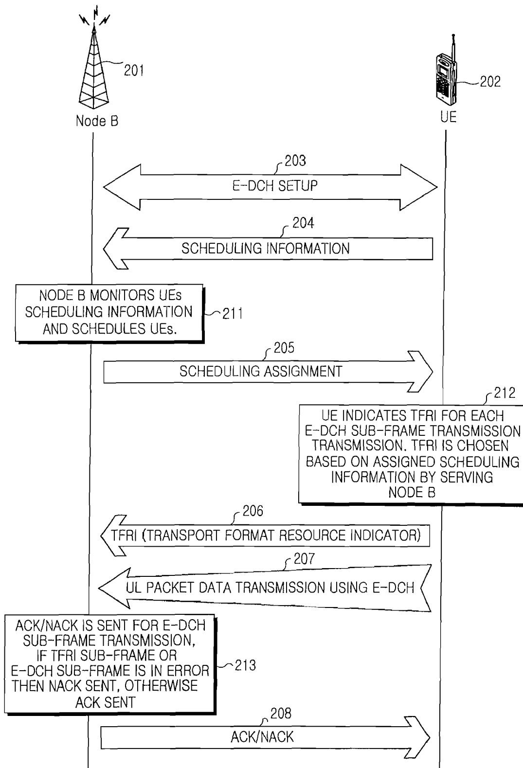
FIG.2 (RELATED ART)
