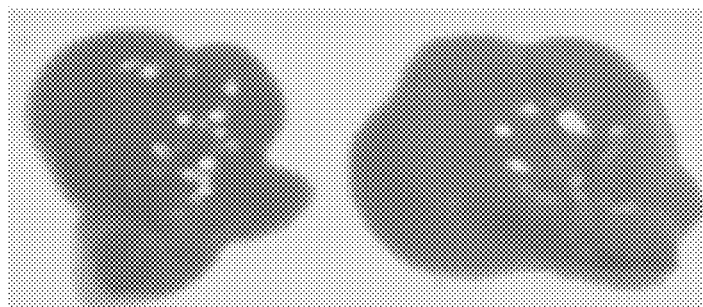
Fatostatin A
