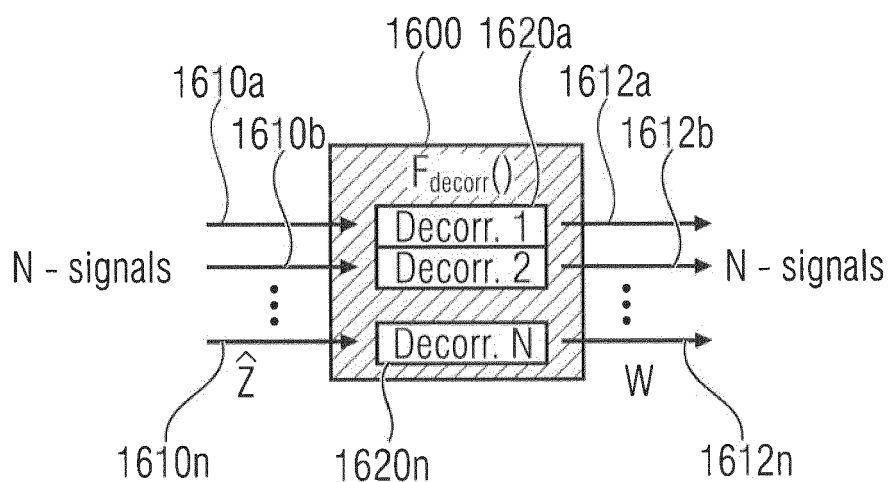
DECORRELATAION UNIT
