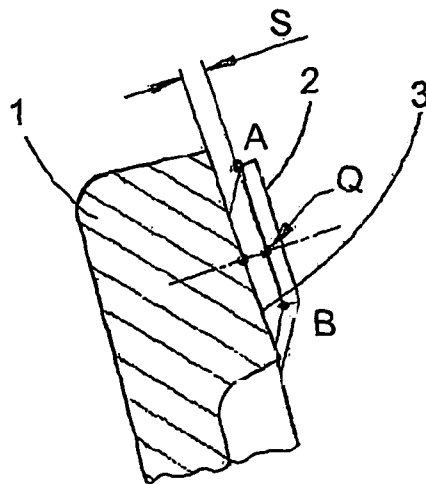
Fig. 3 (SECTION XX)
