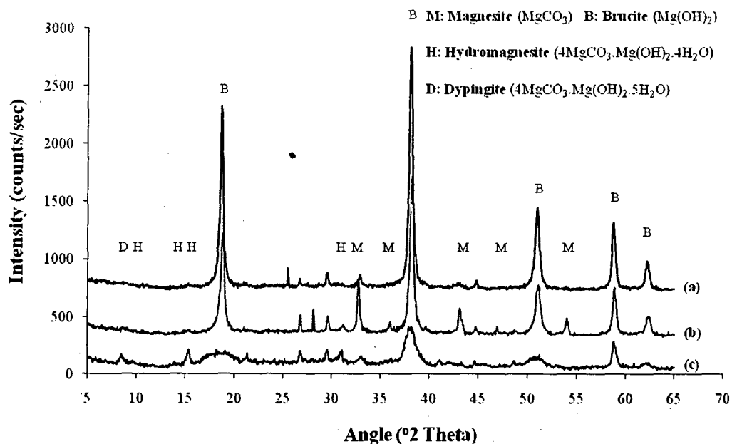
Figure 1 shows the x-ray diffraction spectra of hydrated (a) 100% MgO, (b) 80% MgO - 20% \text{MgCO}_3 and (c) 80% MgO - 20% hydromagnesite samples.
