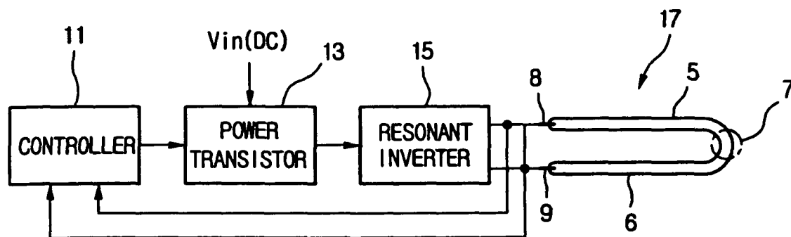
Fig.2 Related Art
