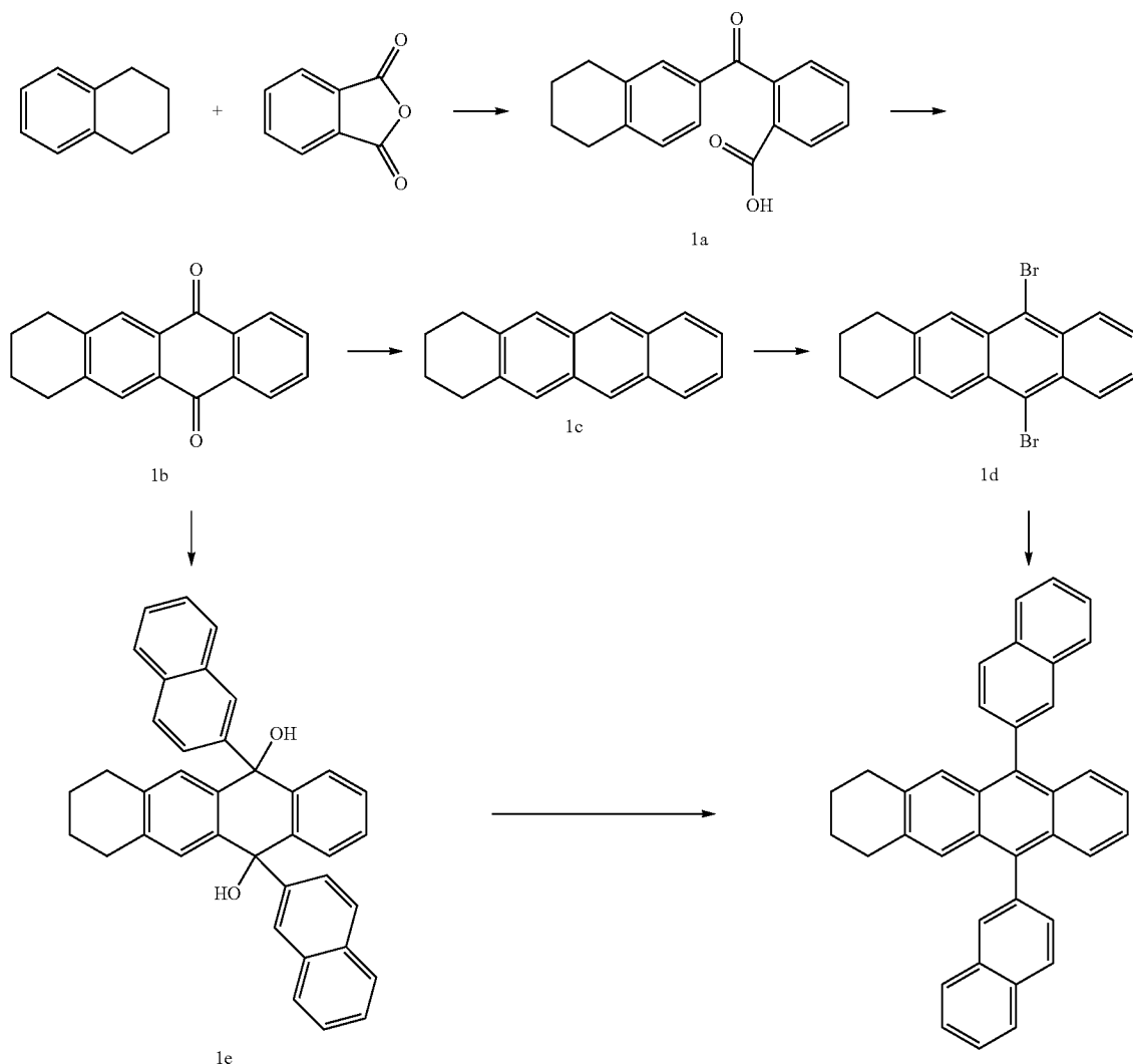
[Reaction scheme 1]
