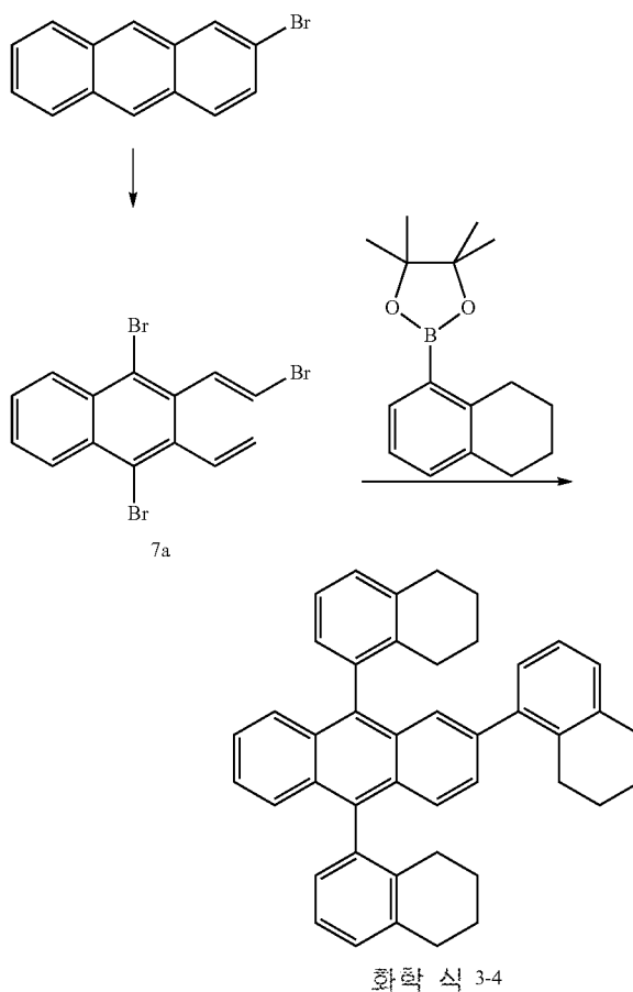
[Reaction scheme 7]
