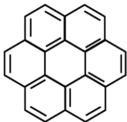
Corene
