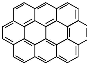
Ovalene
