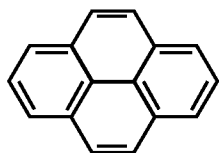
Pyrene
