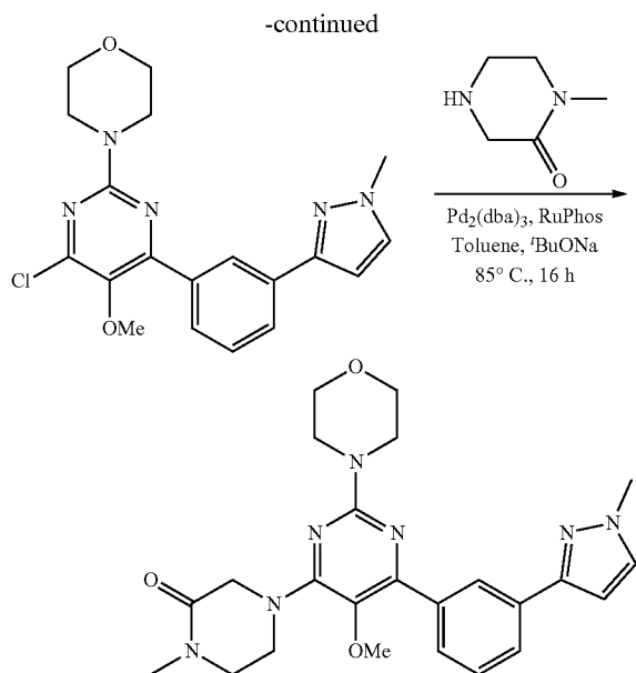
Step 1: Synthesis of 4-(4-chloro-5-methoxy-6-(3-(1-methyl-1H-pyrazol-3-yl)phenyl)pyrimidin-2-yl)morpholine
