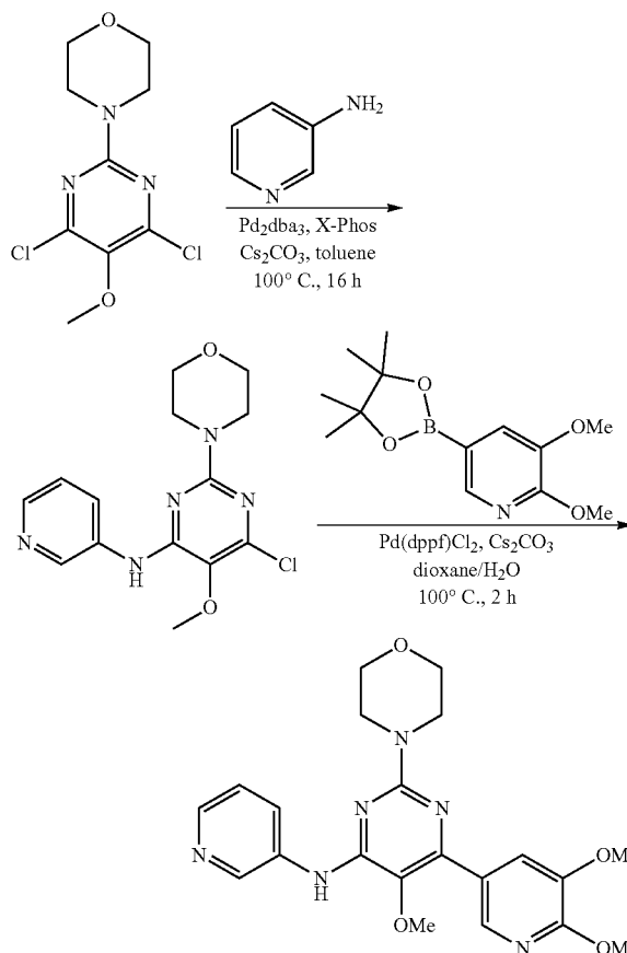
Step 1: Synthesis of 6-chloro-5-methoxy-2-morpholino-N-(pyridin-3-yl)pyrimidin-4-amine
