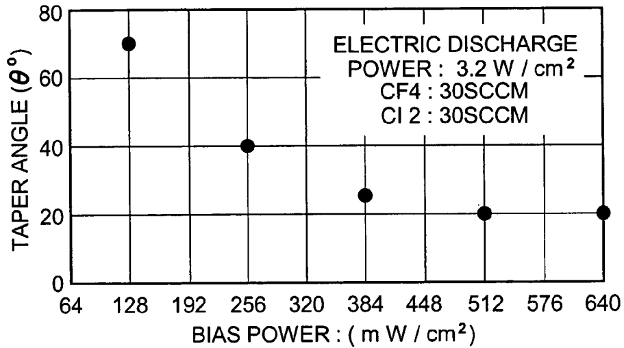
DEPENDENCE OF TAPER ANGLE ON BIAS POWER
