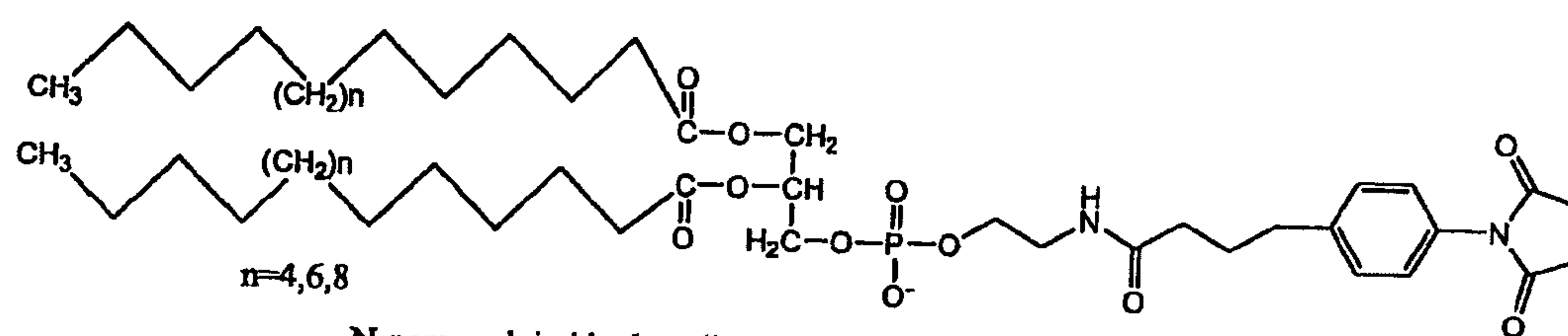
N-para-maleimidophenylbutyrate phosphatidyl ethanolamine
