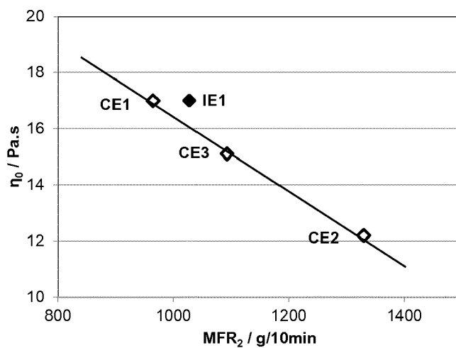
Fig. 1: Correlation between the MFR (230°C / 2.16 kg) and zero shear viscosity for inventive and comparative examples
