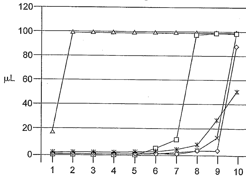
Comparison of Leakage for Syringe-based ID Devices: 21ga 28° bevel
