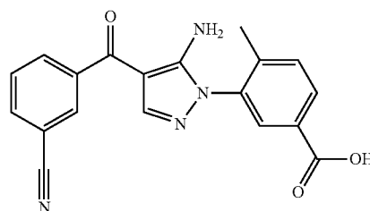
(3-[5-Amino-4-(3-Cyanobenzoyl)-1H-Pyrazol-1-yl]-4-Methylbenzoic Acid)
