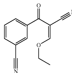
(3-[2-Cyano-2-(Ethoxymethylidene)Acetyl]Benzoni-trile)
