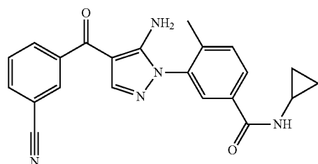
(3-[5-Amino-4-(3-Cyanobenzoyl)-Pyrazol-1-yl]-N-Cyclopropyl-4-Methylbenzamide)
