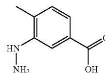
(3-hydrazino-4-methyl-benzoic acid)
