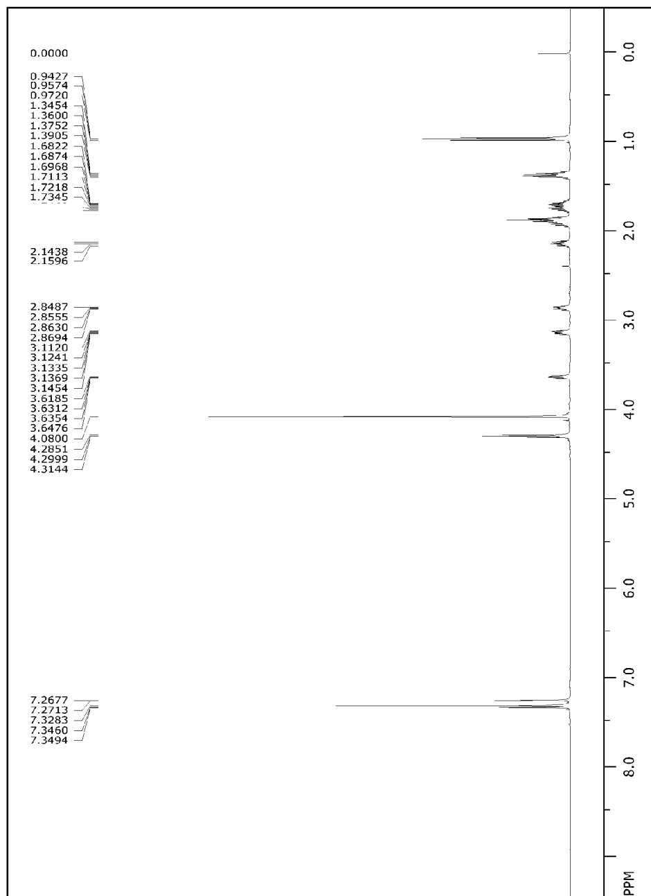
Figure 4 - ^1\text{H} NMR spectrum of 1-Butyl-3-Methylimidazolium Prolinate ( \text{CDCl}_3 , 500 MHz)
