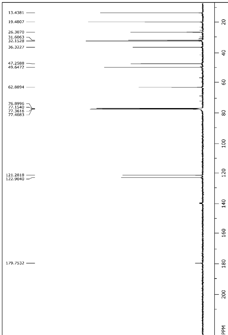
Figure 5 - ^{13}\text{C} NMR spectrum of 1-Butyl-3-Methylimidazolium Proline (CDCl 3 , 125 MHz)
