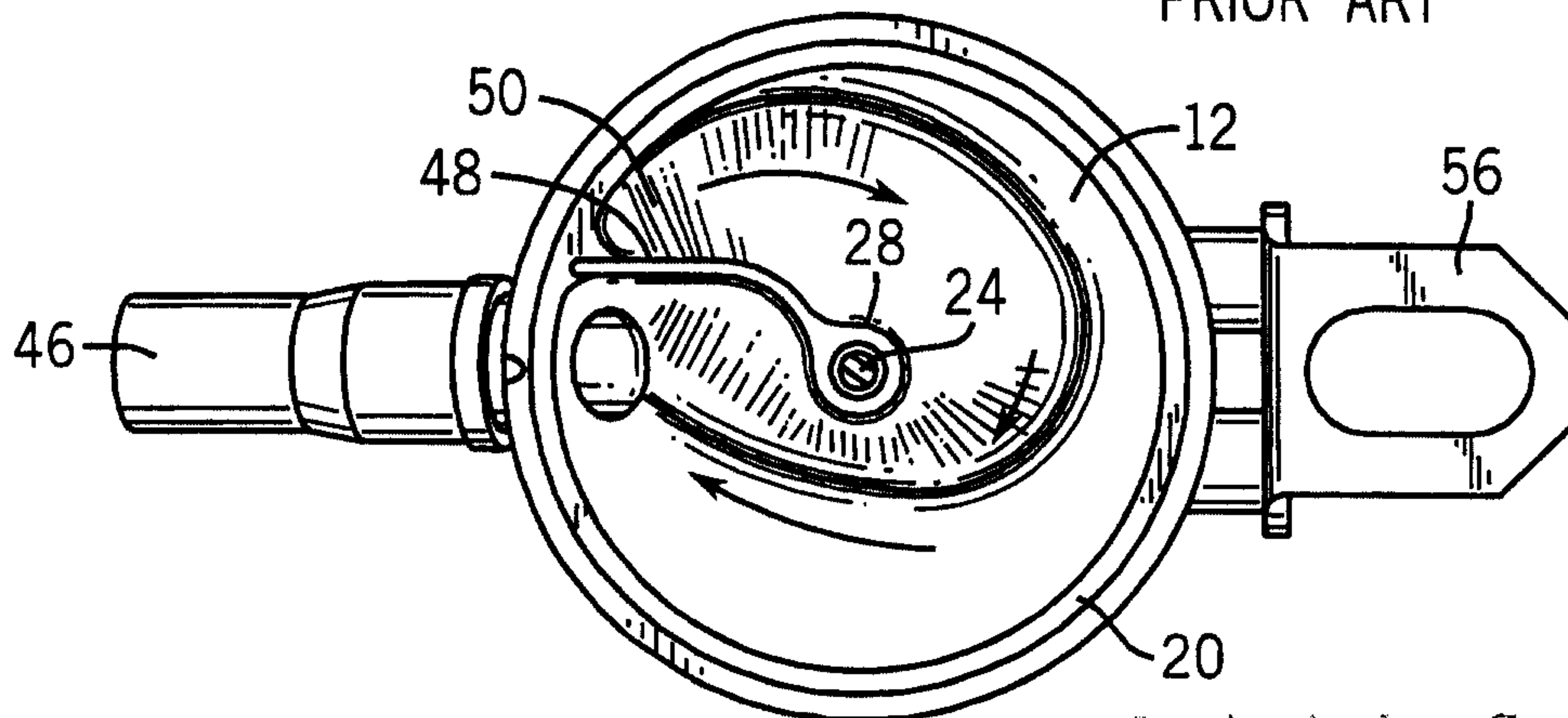
FIG. 5 PRIOR ART
