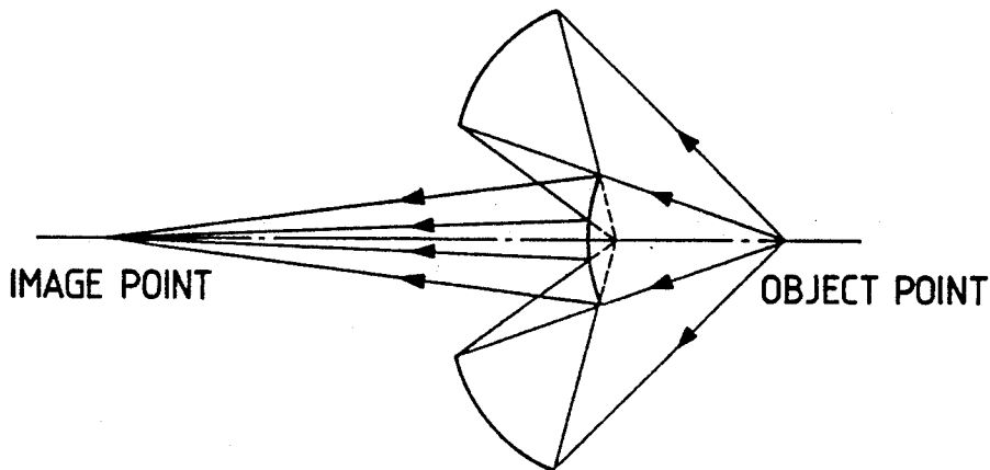
FIG. 3 PRIOR ART
