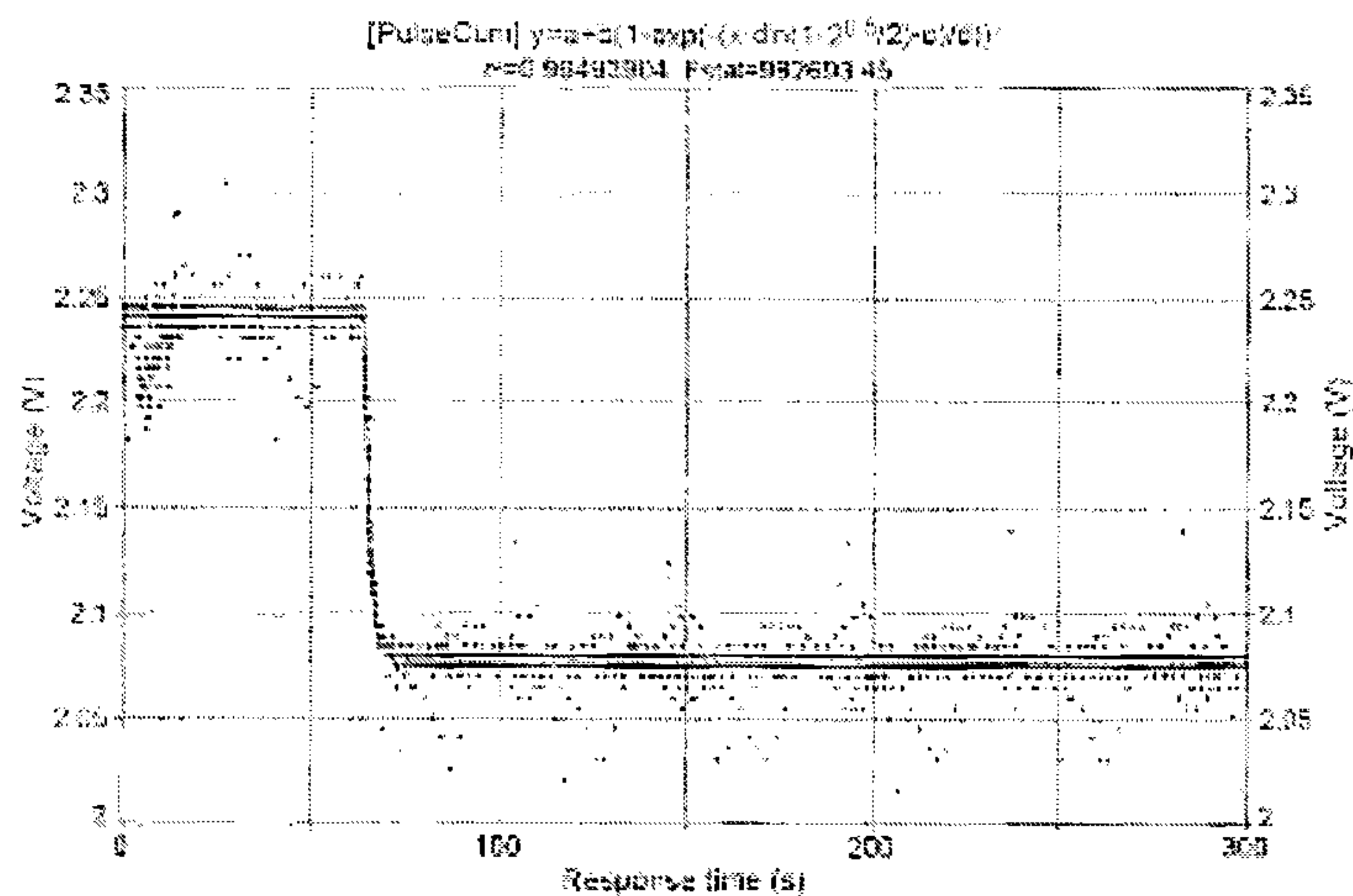
FIGURE 6.40 TYPICAL DATA OF pH PROBE RESPONSE TIME TO A pH STEP CHANGE OF ~0.6. THE RESPONSE WAS FITTED USING TABLECURVE SOFTWARE. THE BEST-FIT PULSE FUNCTION HAD A COEFFICIENT OF CORRELATION OF 0.995.
