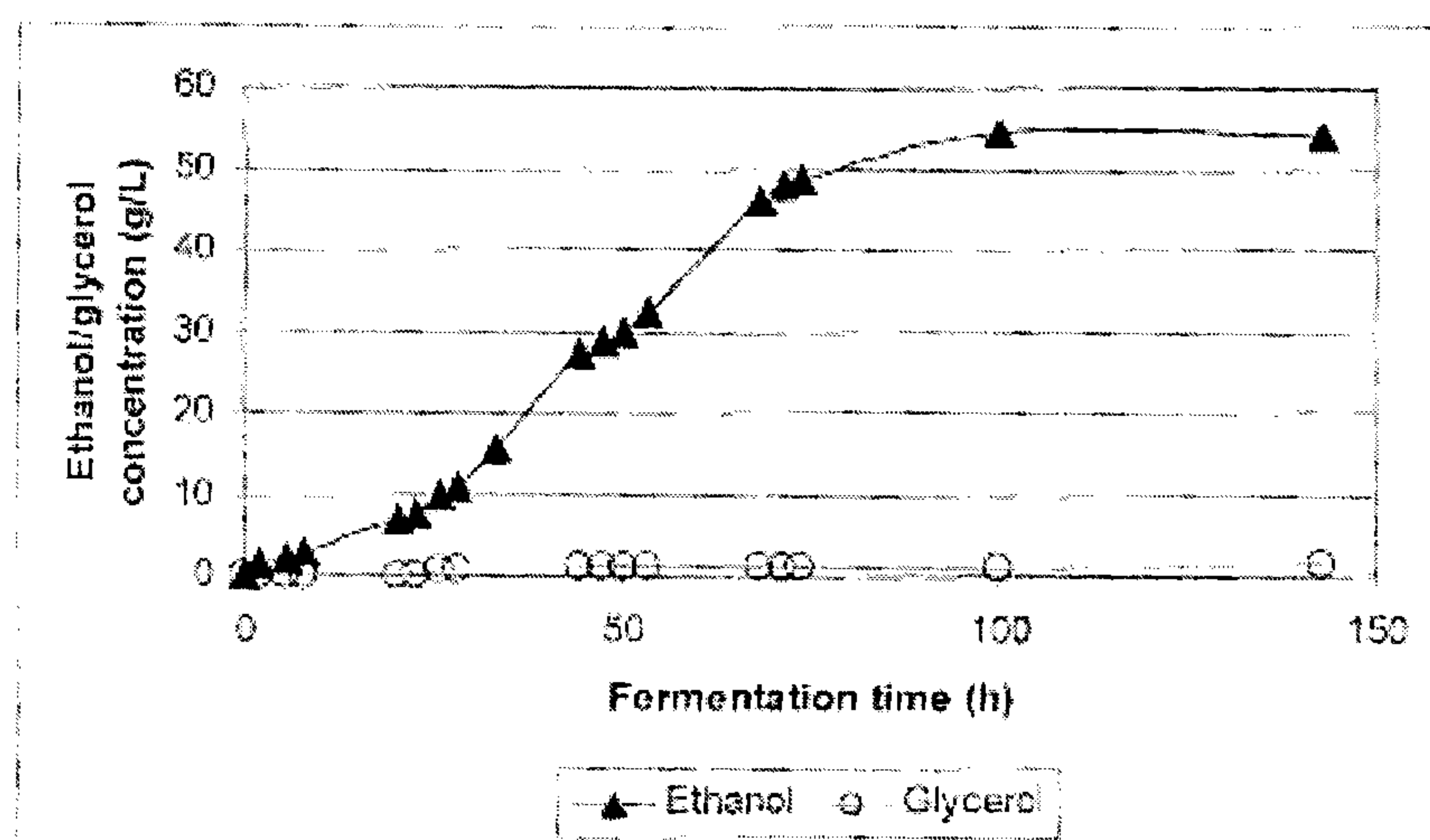
FIGURE 6.5 ETHANOL AND GLYCEROL CONCENTRATIONS VERSUS FERMENTATION TIME FOR LCC3021 YEAST BATCH FERMENTATION 1 WITHIN A PILOT SCALE GLBT BIOREACTOR.
