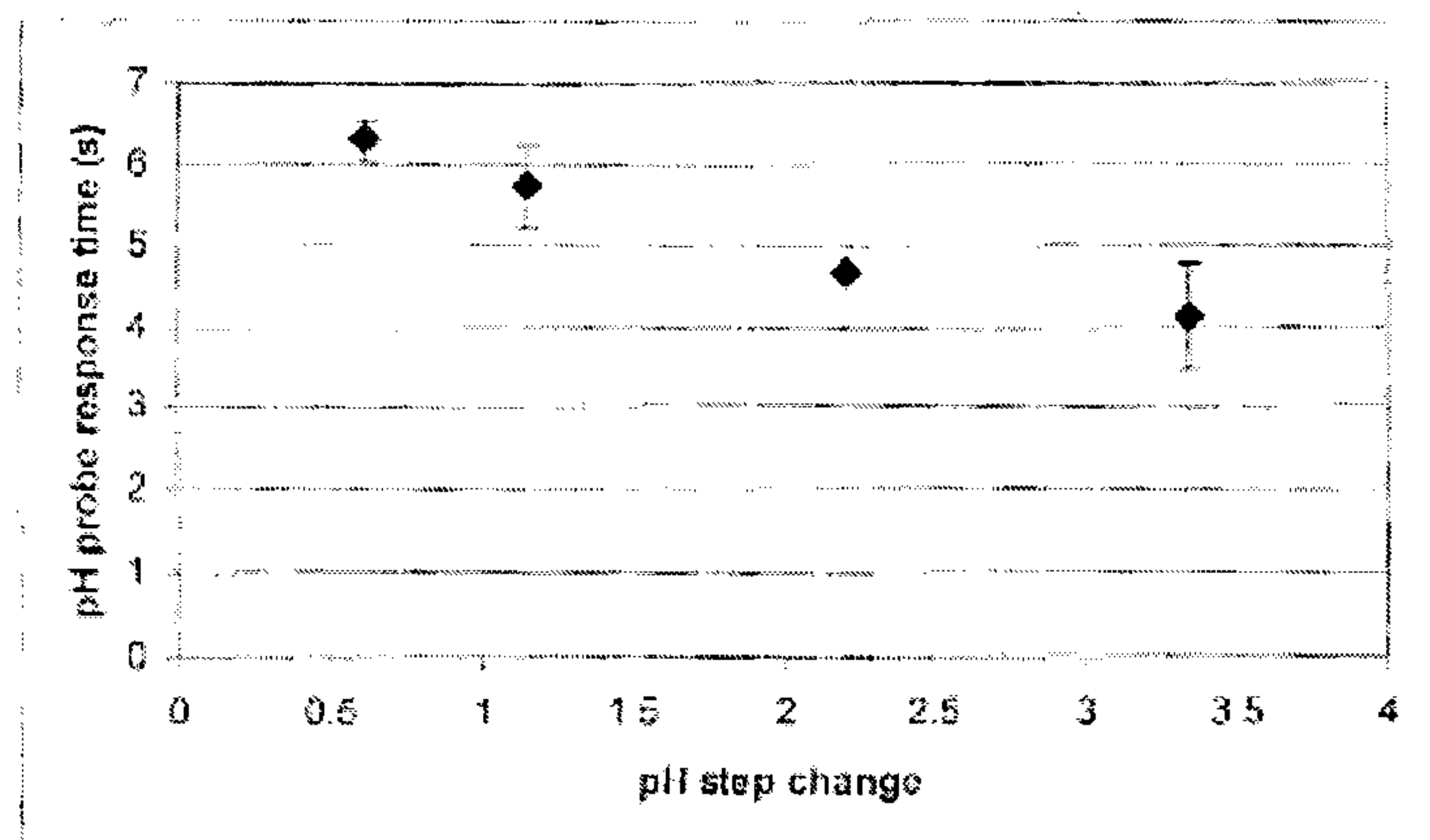
FIGURE 6.44 INGOLD PH PROBE RESPONSE TIME TO A STEP CHANGE. ( n = 3 ) THE PROBE WAS IMMERSSED IN THE HIGHER PH BUFFER THEN IMMEDIATELY SUBJECTED TO THE LOWER PH BUFFER OF 4.0. THE LINE OF BEST FIT FOR EACH RESPONSE CURVE WAS UTILIZED TO CALCULATE THE TIME NECESSARY FOR THE PROBE TO REACH 98% OF THE STEP CHANGE.
