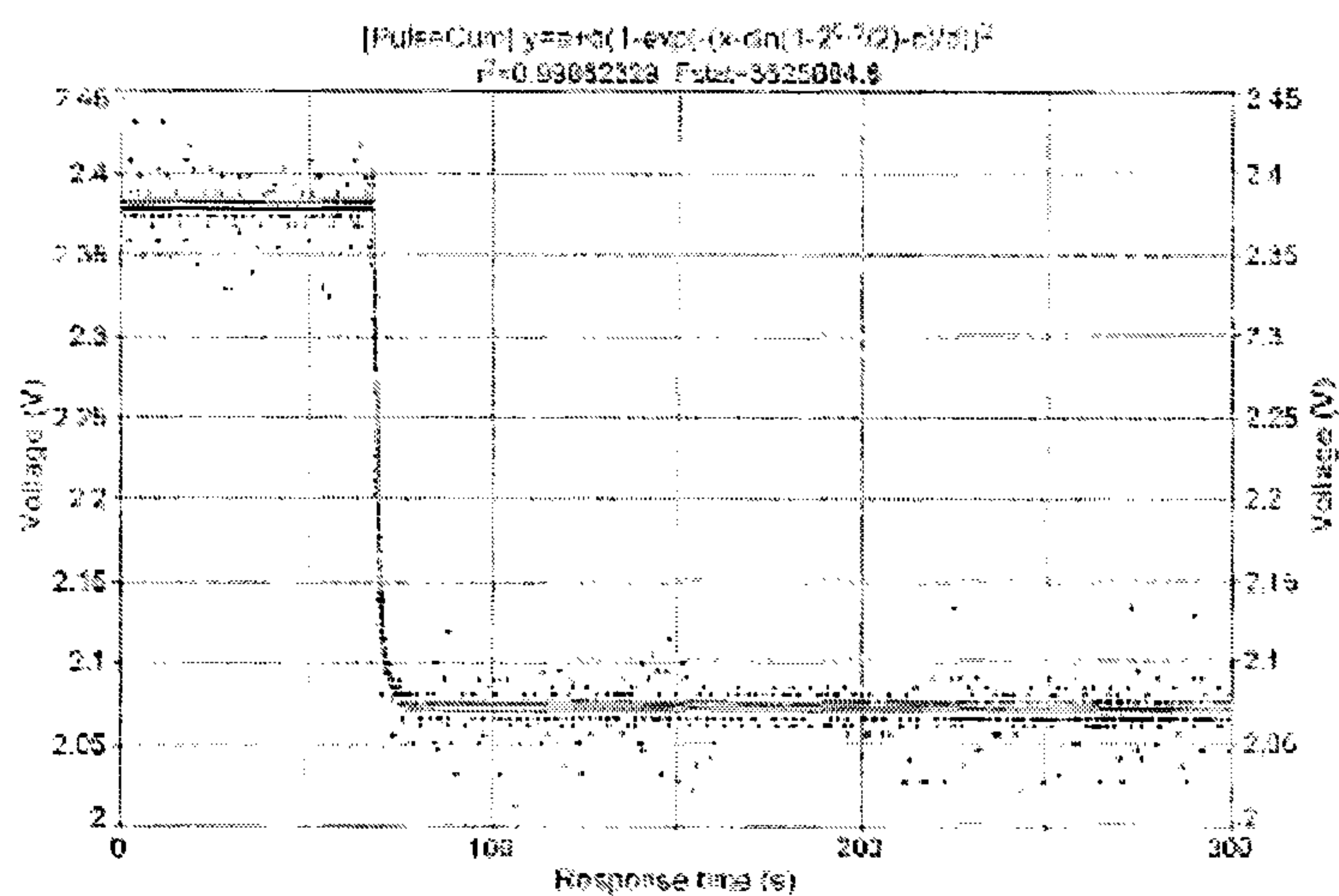
FIGURE 6.41 TYPICAL DATA OF pH PROBE RESPONSE TIME TO A pH STEP CHANGE OF ~1.2. THE RESPONSE WAS FITTED USING TABLECURVE SOFTWARE. THE BEST-FIT PULSE FUNCTION HAD A COEFFICIENT OF CORRELATION OF 0.999.
