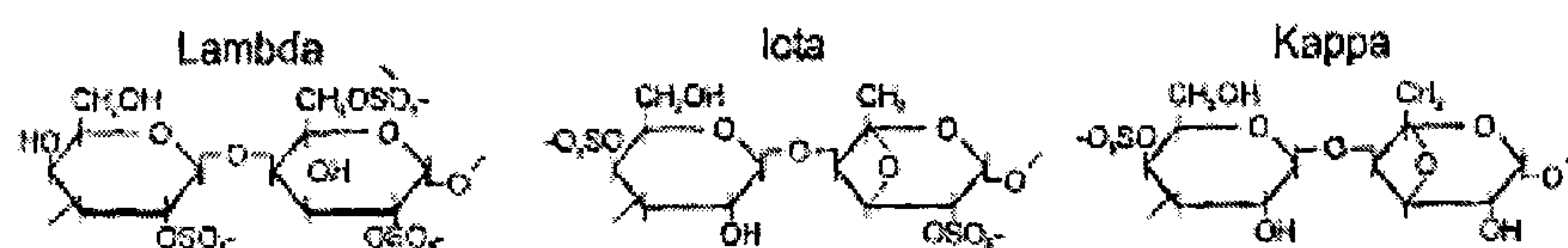
FIGURE 6.2a CHEMICAL STRUCTURES OF LAMBDA-, IOTA- AND KAPPA-CARRAGEENANS
