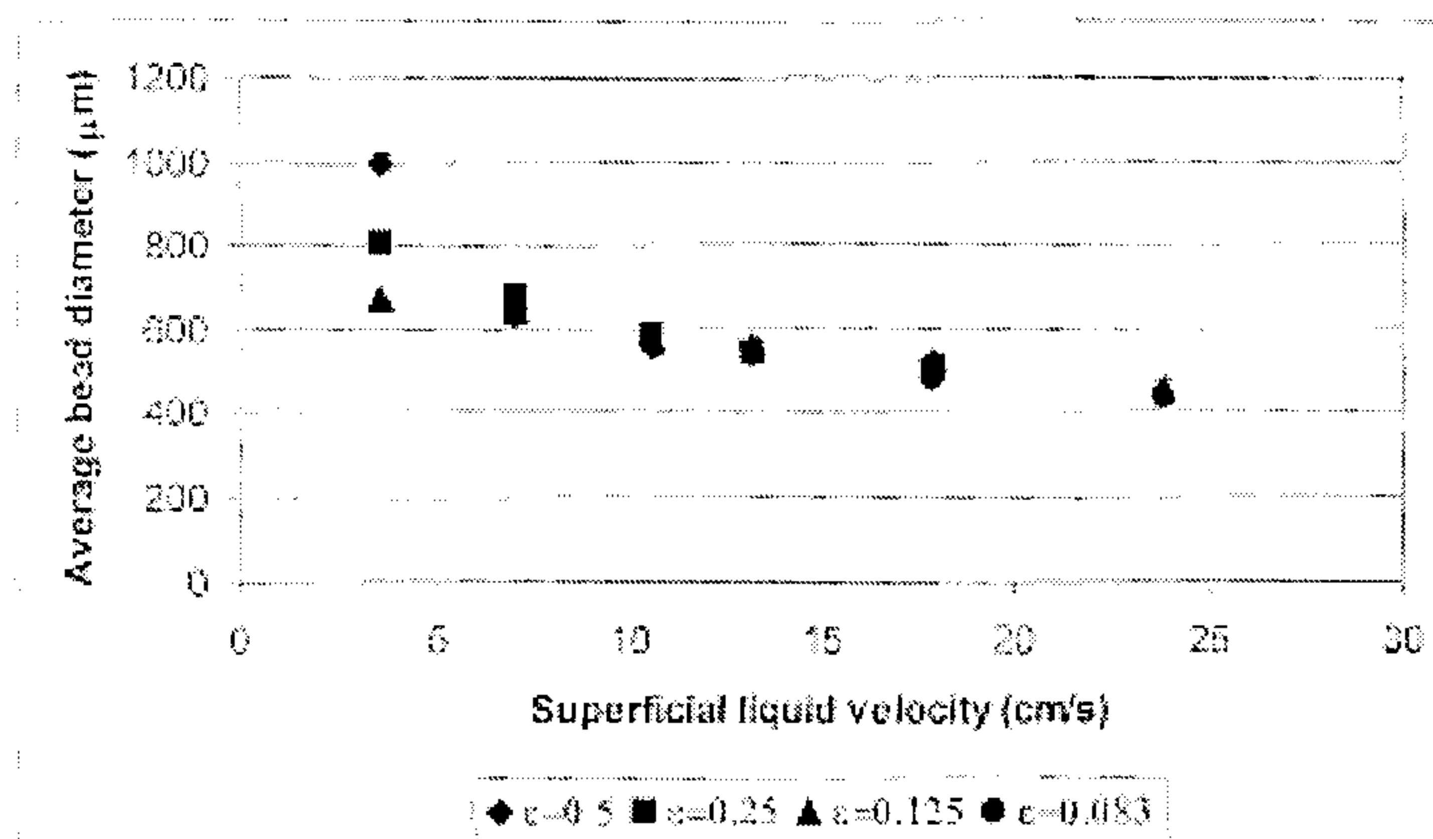
FIGURE 6.16. SUPERFICIAL LIQUID VELOCITY (CM/S) VERSUS AVERAGE BEAD DIAMETER (μM). FOUR POLYMER FRACTIONS ( \phi OF 0.5, 0.25, 0.125 AND 0.083) WERE EVALUATED. THE NUMBER OF STATIC MIXER ELEMENTS ( N_s ) WAS KEPT CONSTANT AT 48 AND THE STATIC MIXER DIAMETER ( D_s ) WAS SET AT 12.7 MM.
