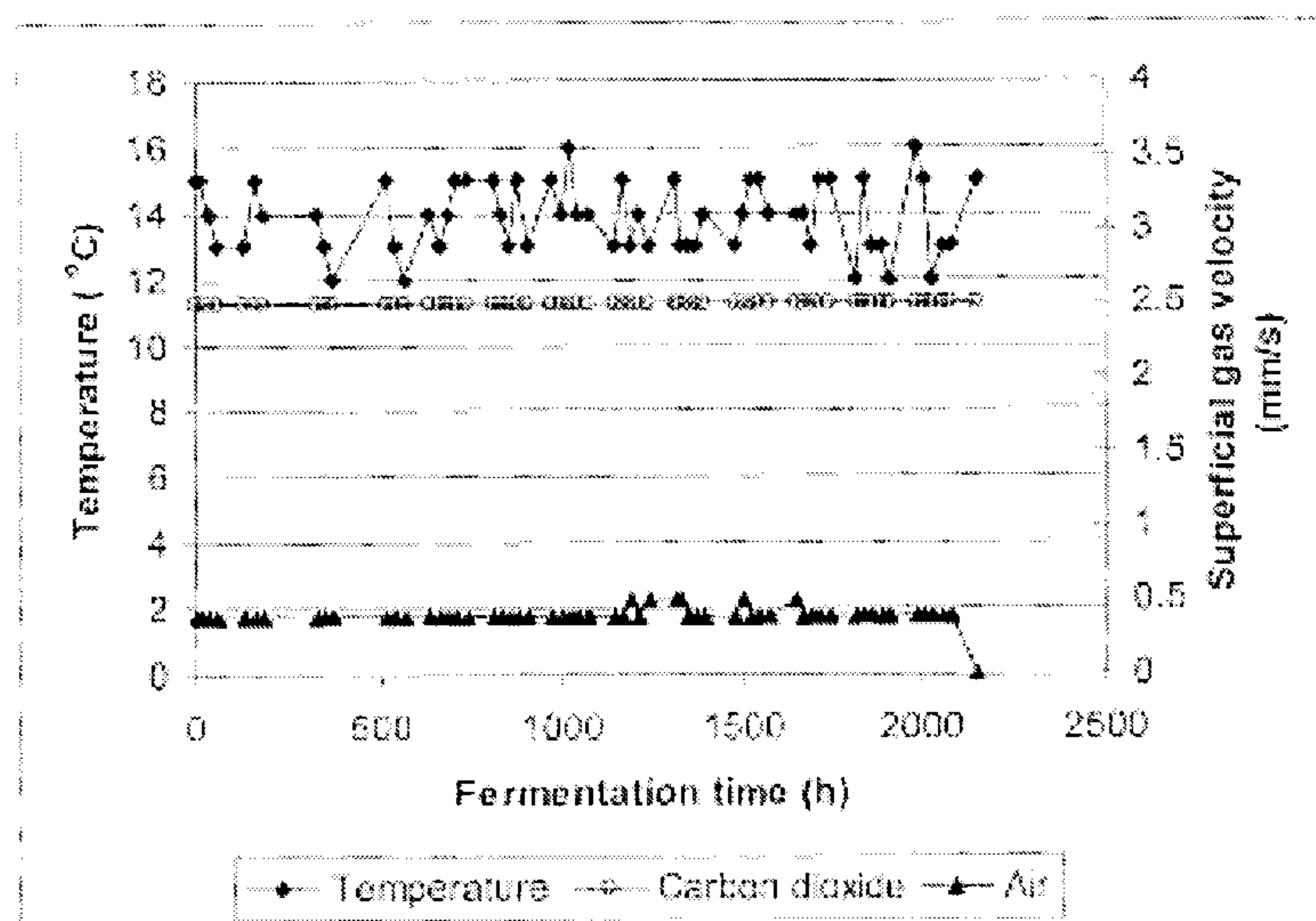
FIGURE 6.69 OPERATING PARAMETER FOR THE LCC302L FERMENTATION VERSUS FERMENTATION TIME.
