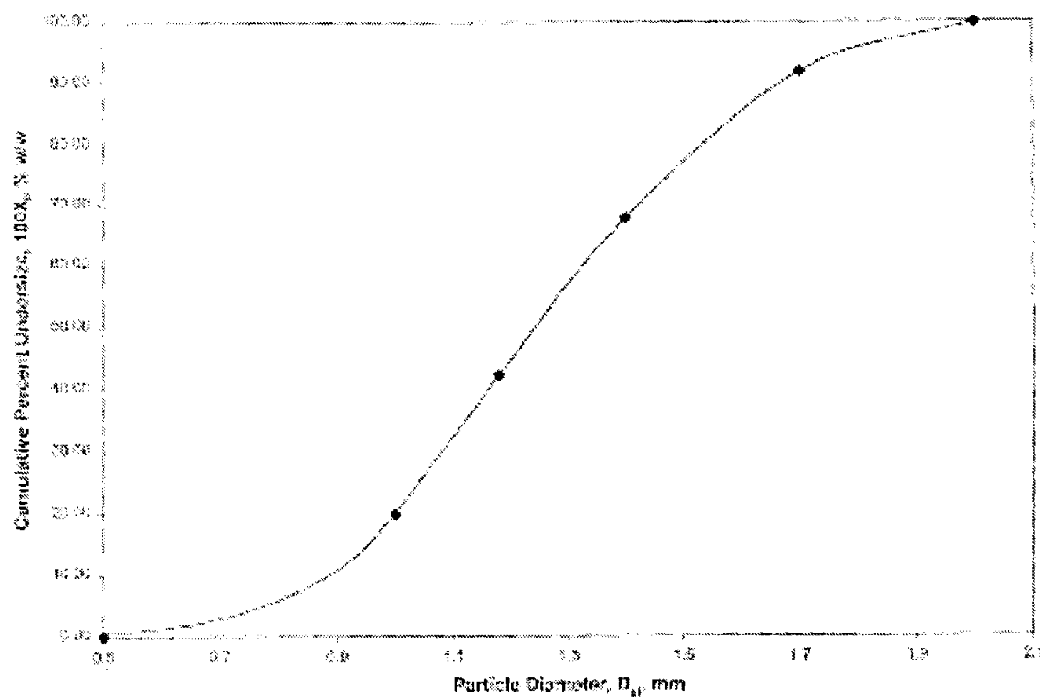
FIGURE 5.8a CUMULATIVE PARTICLE SIZE DISTRIBUTION OF KAPPA-CARRAGEENAN GEL BEADS CONTAINING IMMOBILIZED YEAST CELLS (N=5)
