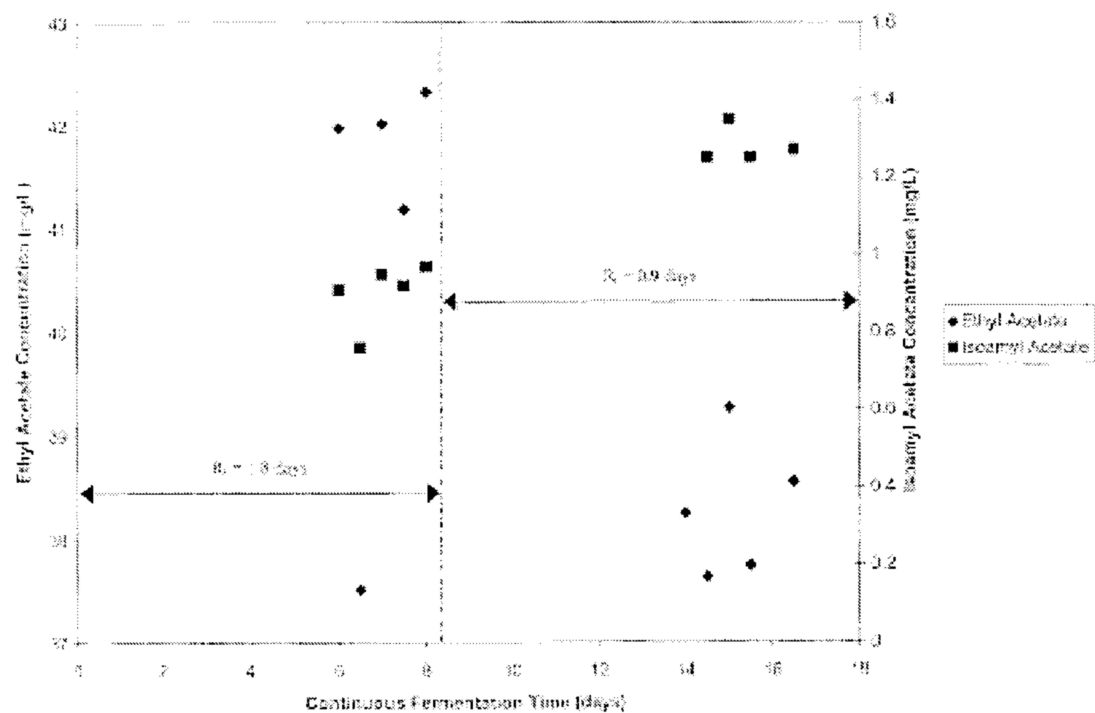
FIGURE 7.28. LIQUID PHASE ETHYL ACETATE AND ISOAMYL ACETATE CONCENTRATION VERSUS RELATIVE CONTINUOUS FERMENTATION TIME, EFFECT OF LIQUID RESIDENCE TIME IN BIOREACTOR. R_t IS BIOREACTOR LIQUID RESIDENCE TIME IN DAYS.
