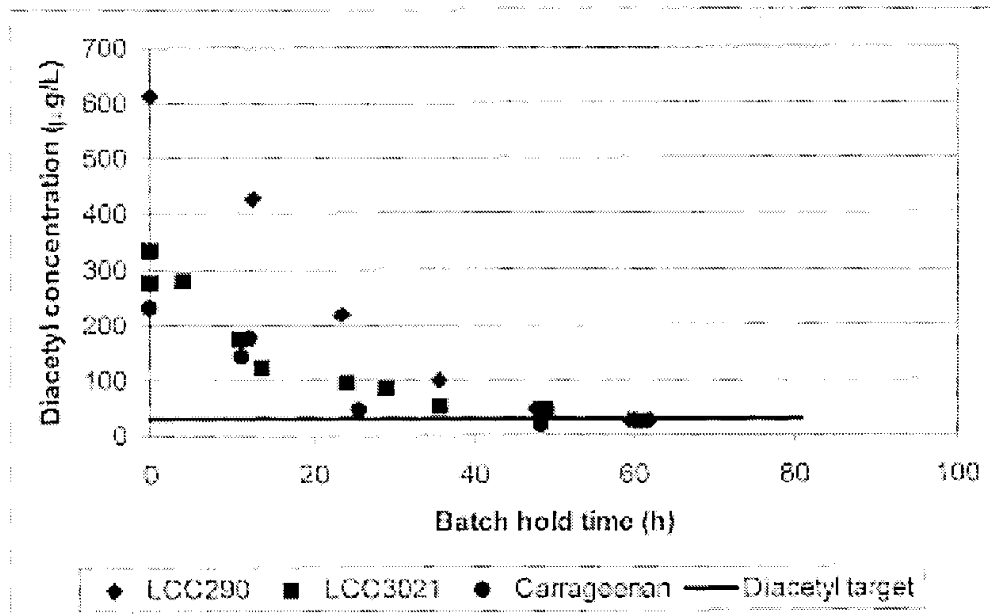
FIGURE 6.78 DIACETYL CONCENTRATION VERSUS WARM BATCH HOLD FOLLOWING CONTINUOUS PRIMARY FERMENTATION WITH LCC290 YEAST, LCC3021 YEAST AND CARRAGEENAN GEL IMMOBILIZED YEAST IN THE GAS-LIFT SYSTEM.
