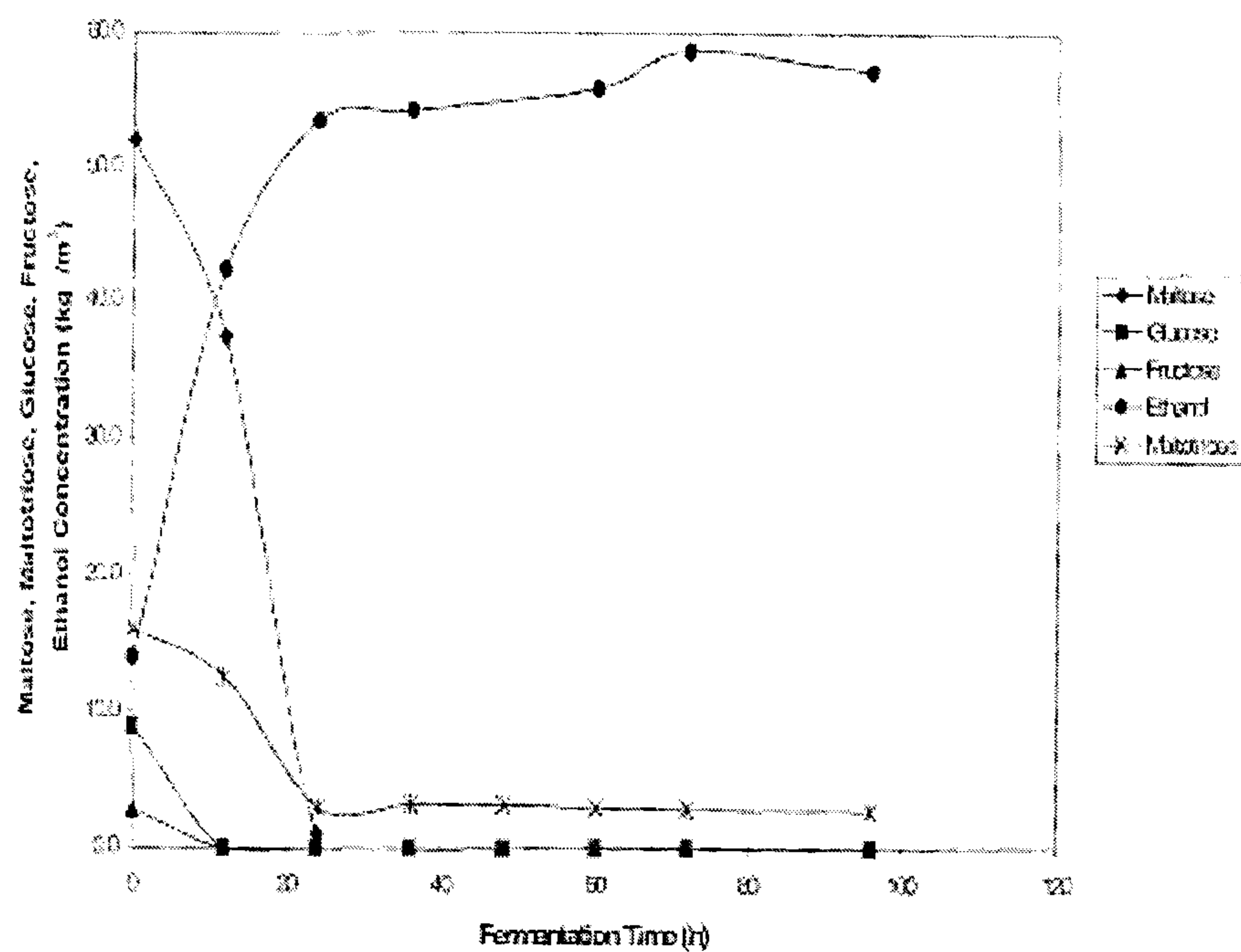
Figure 6.4. c) K 2 , maltose, maltotriose, glucose, fructose, and ethanol concentration versus fermentation time for repeated batch fermentations using S. cerevisiae yeast cells immobilized in kappa-carrageenan gel beads
