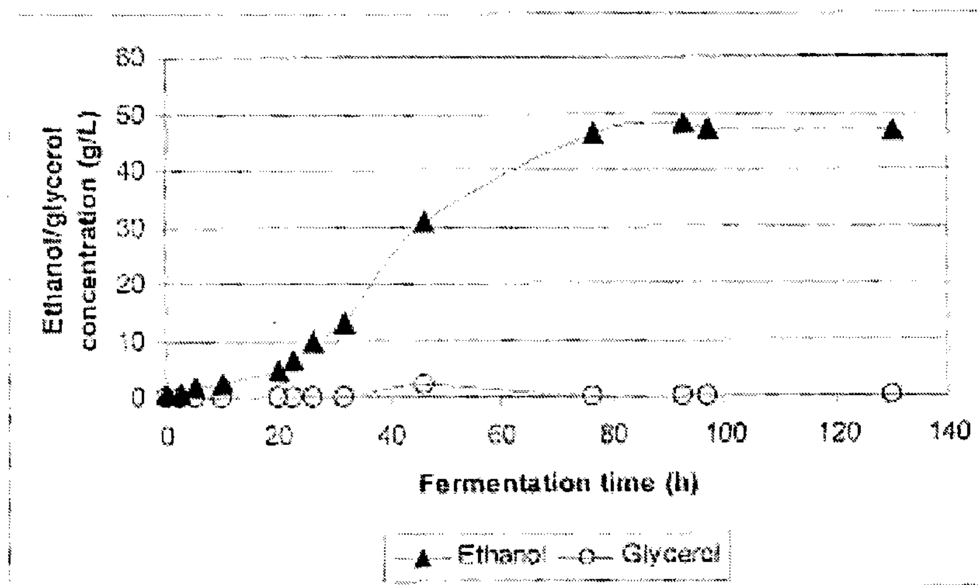
FIGURE 6.6 ETHANOL AND GLYCEROL CONCENTRATIONS VERSUS FERMENTATION TIME FOR LCC3921 YEAST BATCH FERMENTATION 2 WITHIN A PILOT SCALE GLDT BIOREACTOR.
