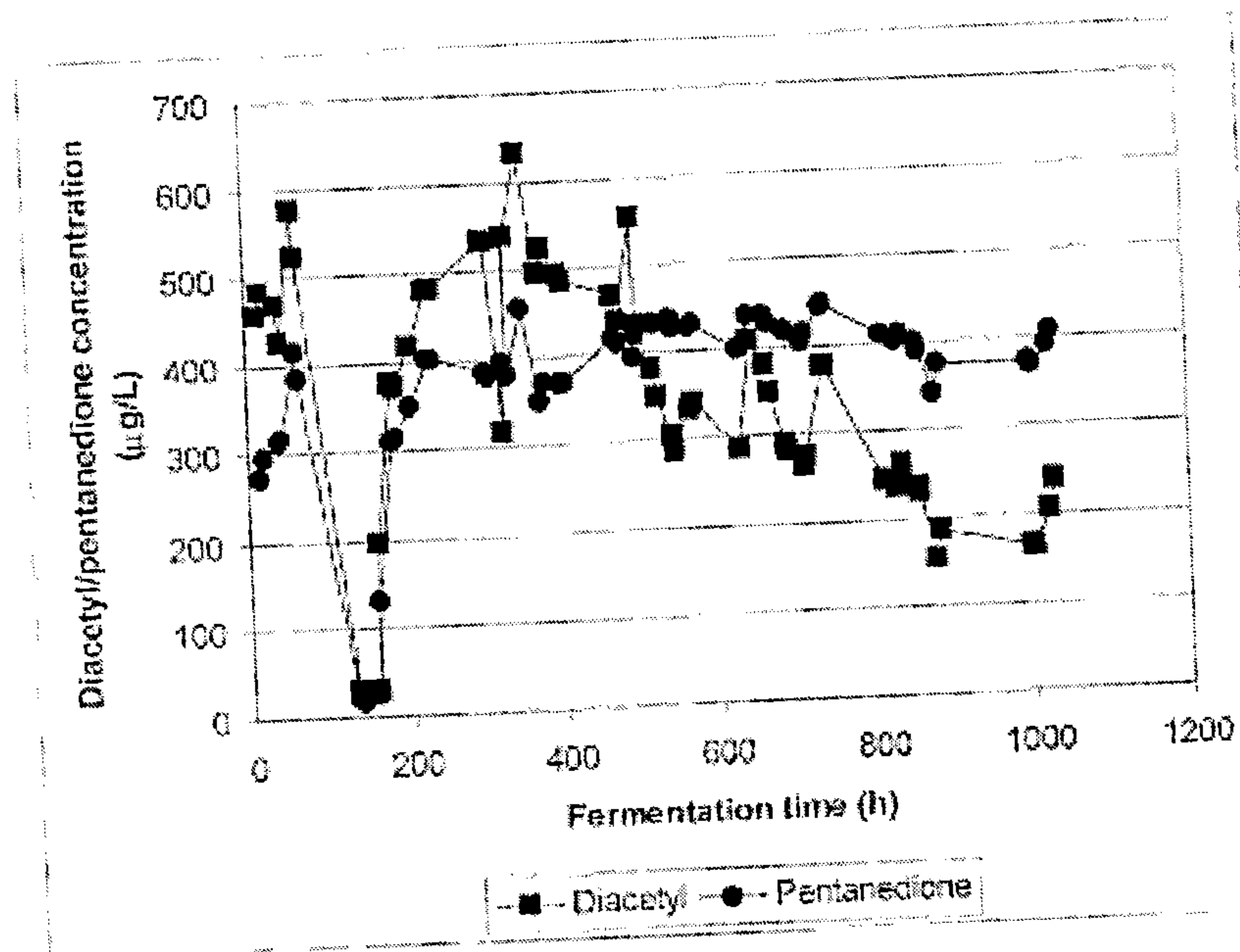
FIGURE 6.63 VICINAL DIKETONES CONCENTRATION OF CARRAGEENAN IMMOBILIZED CONTINUOUS FERMENTATION VERSUS FERMENTATION TIME.
