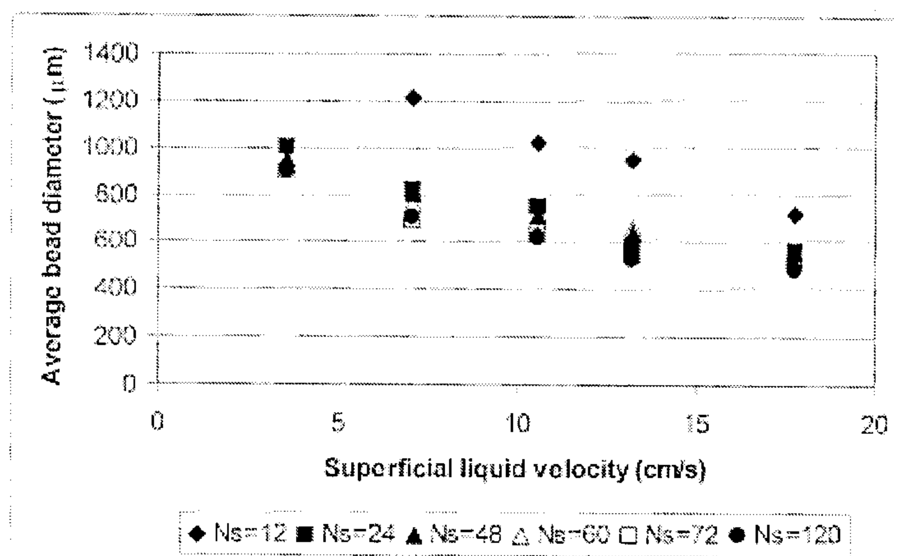
FIGURE 6.18. SUPERFICIAL LIQUID VELOCITY ( \text{cm/s} ) VERSUS AVERAGE BEAD DIAMETER ( \mu\text{m} ). THE NUMBER OF STATIC MIXER ELEMENTS ( N_s ) WAS VARIED TO 12, 24, 48, 60, 72 AND 120. THE POLYMER FRACTION ( \phi_c ) WAS KEPT CONSTANT AT 0.25 AND THE STATIC MIXER DIAMETER ( D_s ) WAS SET AT 12.7 MM.
