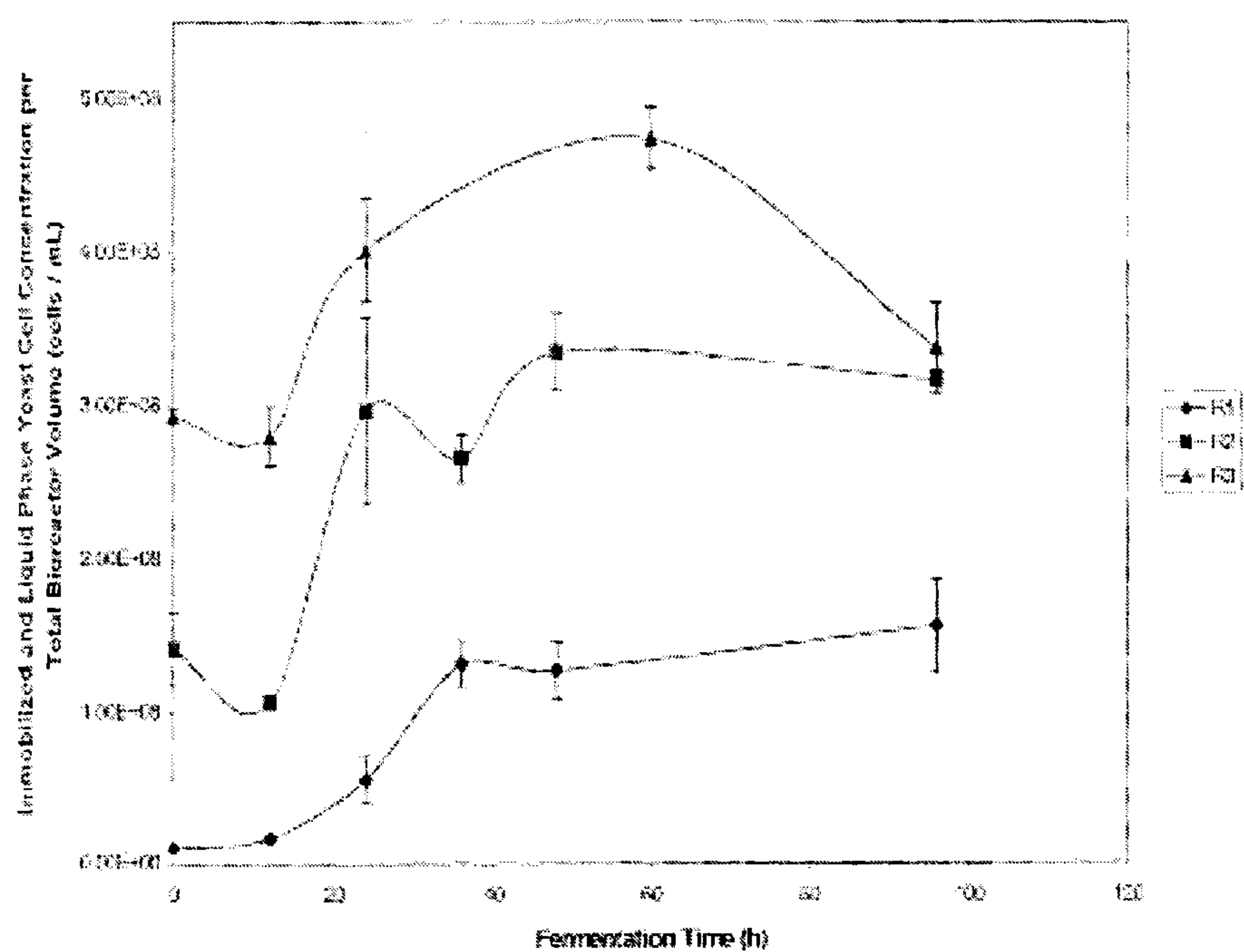
Figure 6.7. b) Concentration per total bioreactor volume of lager yeast cells released into bulk liquid phase versus fermentation time for R1, R2, and R3 fermentations. Error bars represent the upper and lower limits of the experimental data ( n = 2 ).
