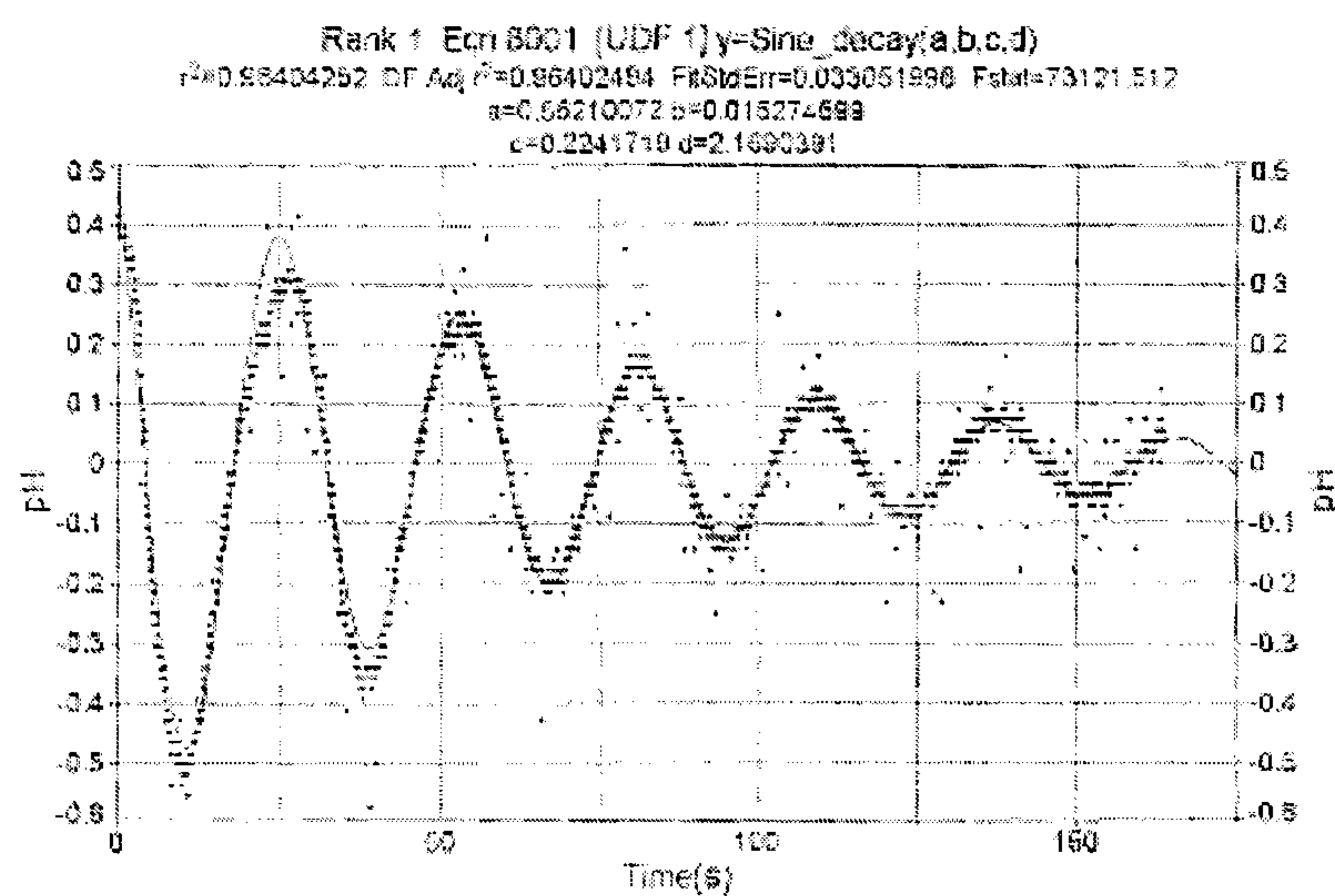
FIGURE 6.44 INGOLD PH PROBE RESPONSE TIME TO A STEP CHANGE. ( n = 3 ) THE PROBE WAS IMMERSSED IN THE HIGHER PH BUFFER THEN IMMEDIATELY SUBJECTED TO THE LOWER PH BUFFER OF 4.0. THE LINE OF BEST FIT FOR EACH RESPONSE CURVE WAS UTILIZED TO CALCULATE THE TIME NECESSARY FOR THE PROBE TO REACH 98% OF THE STEP CHANGE.
