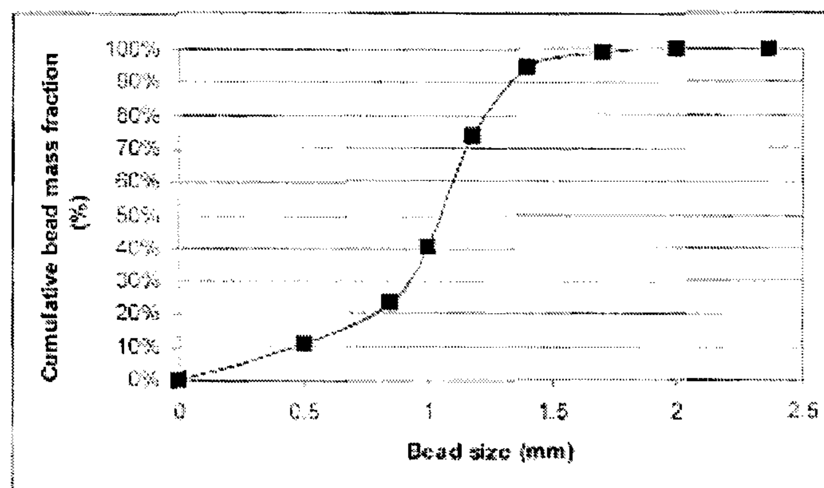
FIGURE 6.24. CUMULATIVE BEAD SIZE DISTRIBUTION OF K-CARRAGEENAN GEL BEADS UTILIZED IN THE CONTINUOUS FERMENTATION TRIALS WITHIN THE 50L GAS-LIFT DRAFT TUBE BIOREACTOR.
