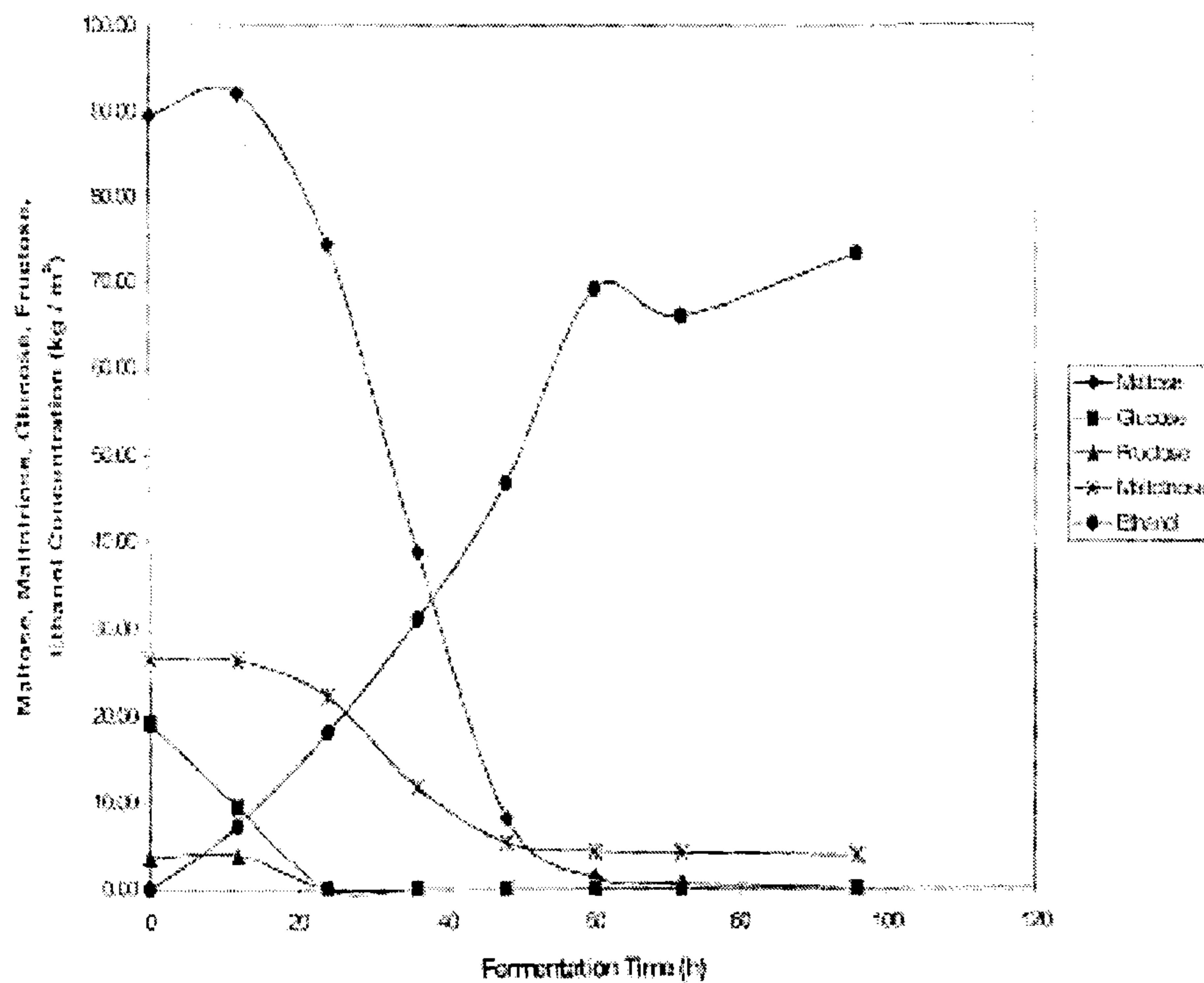
FIGURE 6.5 a MALTOS, MALTOTRIOS, GLUCOS, FRUCTOS, AND ETHANOL CONCENTRATION VERSUS FERMENTATION TIME FOR FREELY SUSPENDED LAGER YEAST CONTROL FERMENTATIONS (NO IMMOBILIZED CELLS)
