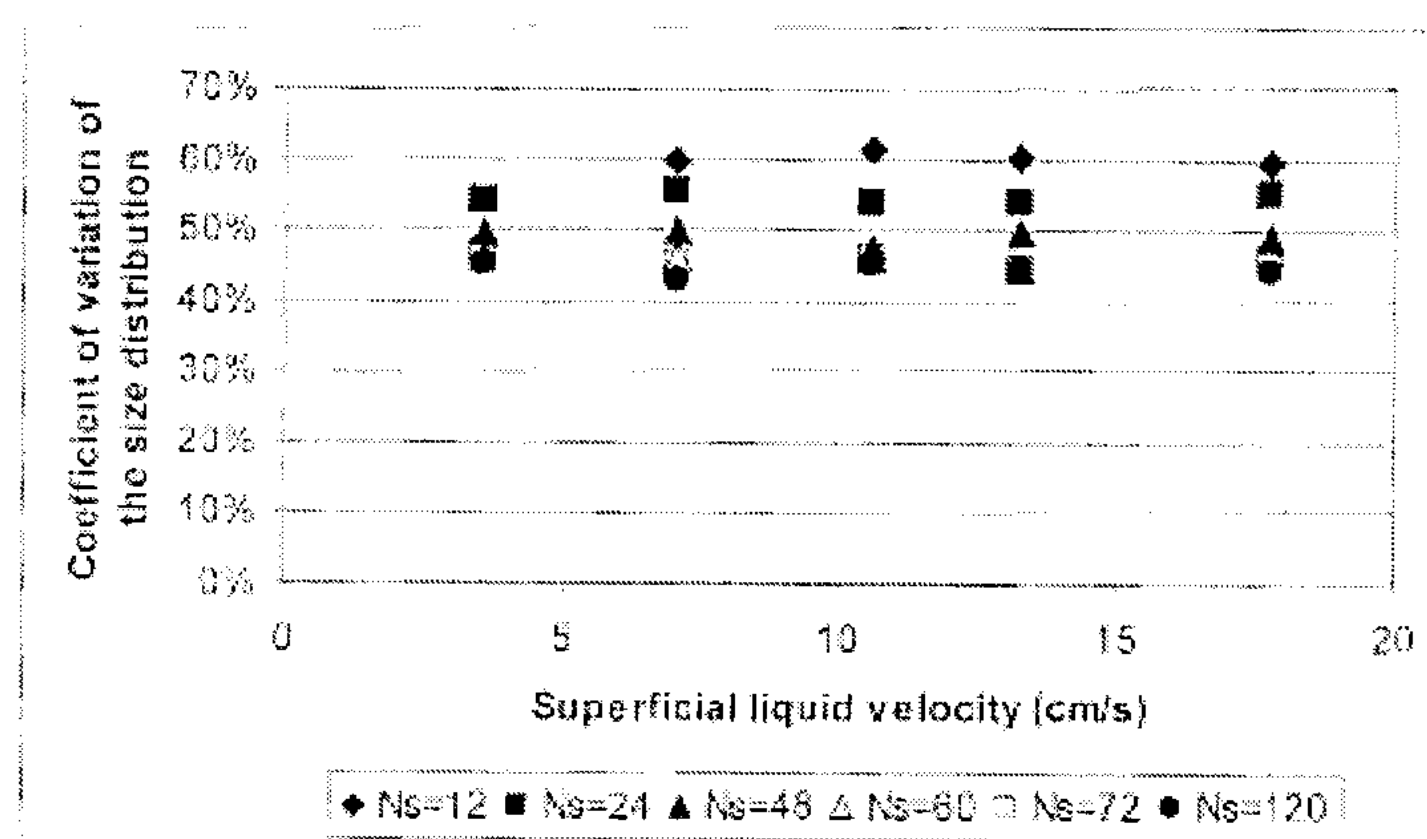
FIGURE 6.19. SUPERFICIAL LIQUID VELOCITY ( \text{cm/s} ) VERSUS COEFFICIENT OF VARIATION OF THE BEAD DIAMETER ( \mu\text{m} ). THE NUMBER OF STATIC MIXER ELEMENTS ( N_s ) WAS VARIED TO 12, 24, 48, 60, 72 AND 120. THE POLYMER FRACTION ( \phi_c ) WAS KEPT CONSTANT AT 0.25 AND THE STATIC MIXER DIAMETER ( D_s ) WAS SET AT 12.7 MM.
