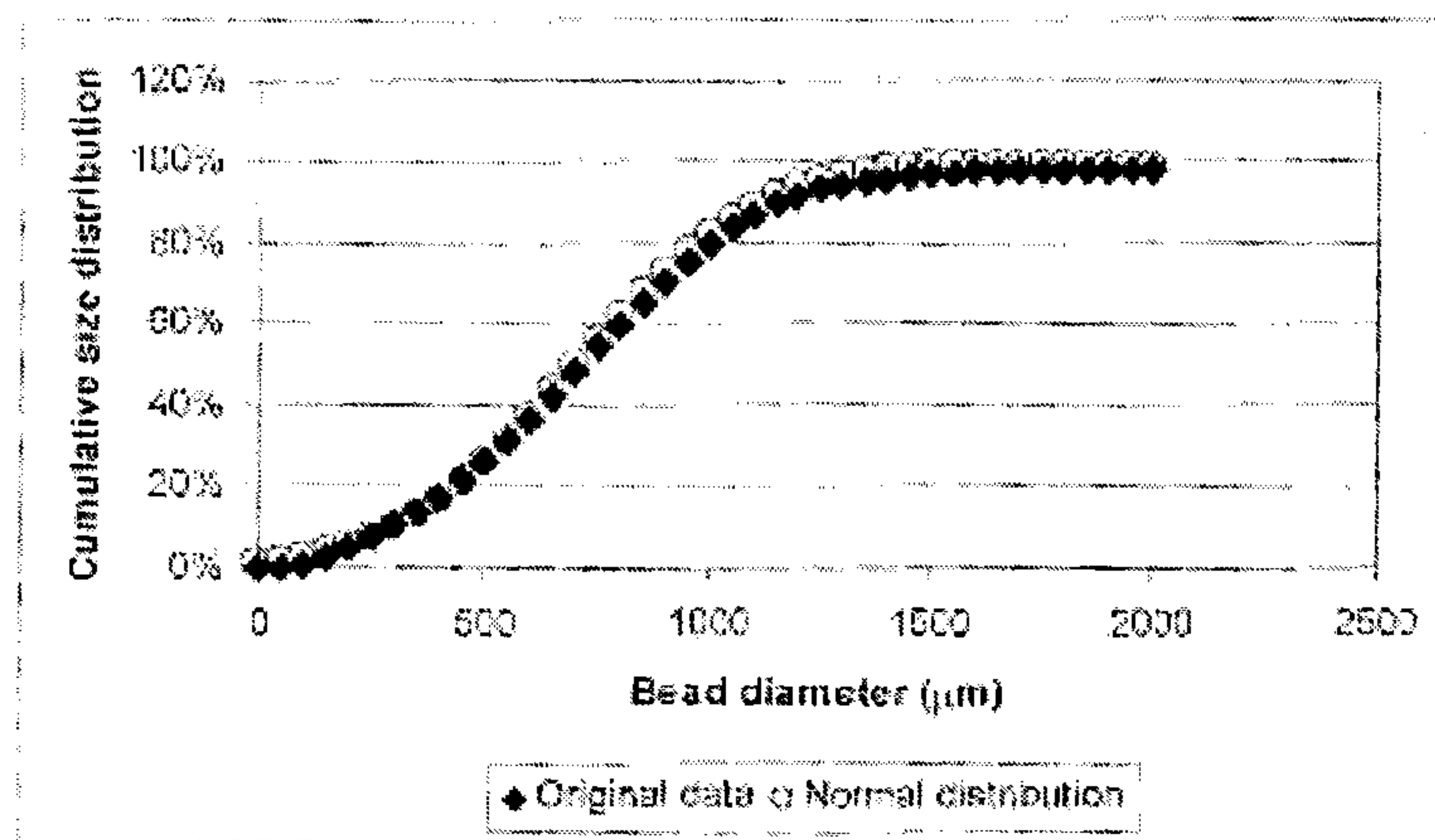
FIGURE 6.13. TYPICAL CUMULATIVE SIZE DISTRIBUTION OF BEADS PRODUCED USING THE STATIC MIXER PROCESS. THE PROCESS PARAMETERS IN THIS EXAMPLE WERE: D_c = 12.7 mm, N_s = 60 , V_{st} = 10.5 cm/s AND U_c = 0.35 .
