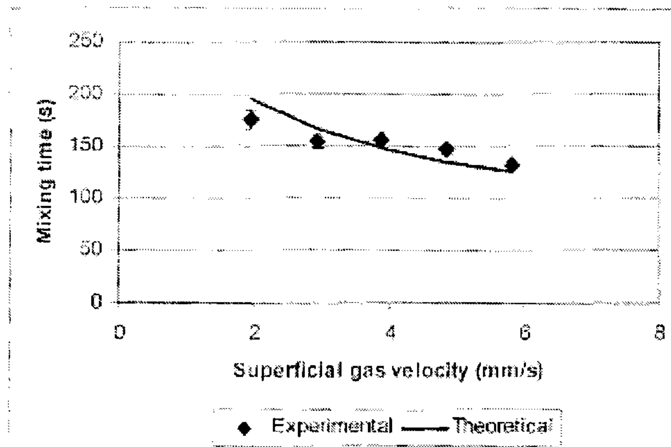
FIGURE 6.51 MIXING TIME VERSUS SUPERFICIAL GAS VELOCITY IN A 50 L GAS-LIFT DRAFT TUBE BIOREACTOR. AN ACID PULSE WAS INJECTED INTO A FERMENTATION MEDIUM CONTAINING YEAST, LCC3021, IMMOBILIZED WITHIN \Gamma -CARRAGEENAN GEL BEADS (BEAD SIZE 1-2 MM). MIXING TIME CORRESPONDS TO THE TIME NECESSARY FOR 98% OF THE STEP CHANGE TO BE NULLIFIED. (N = 3)
