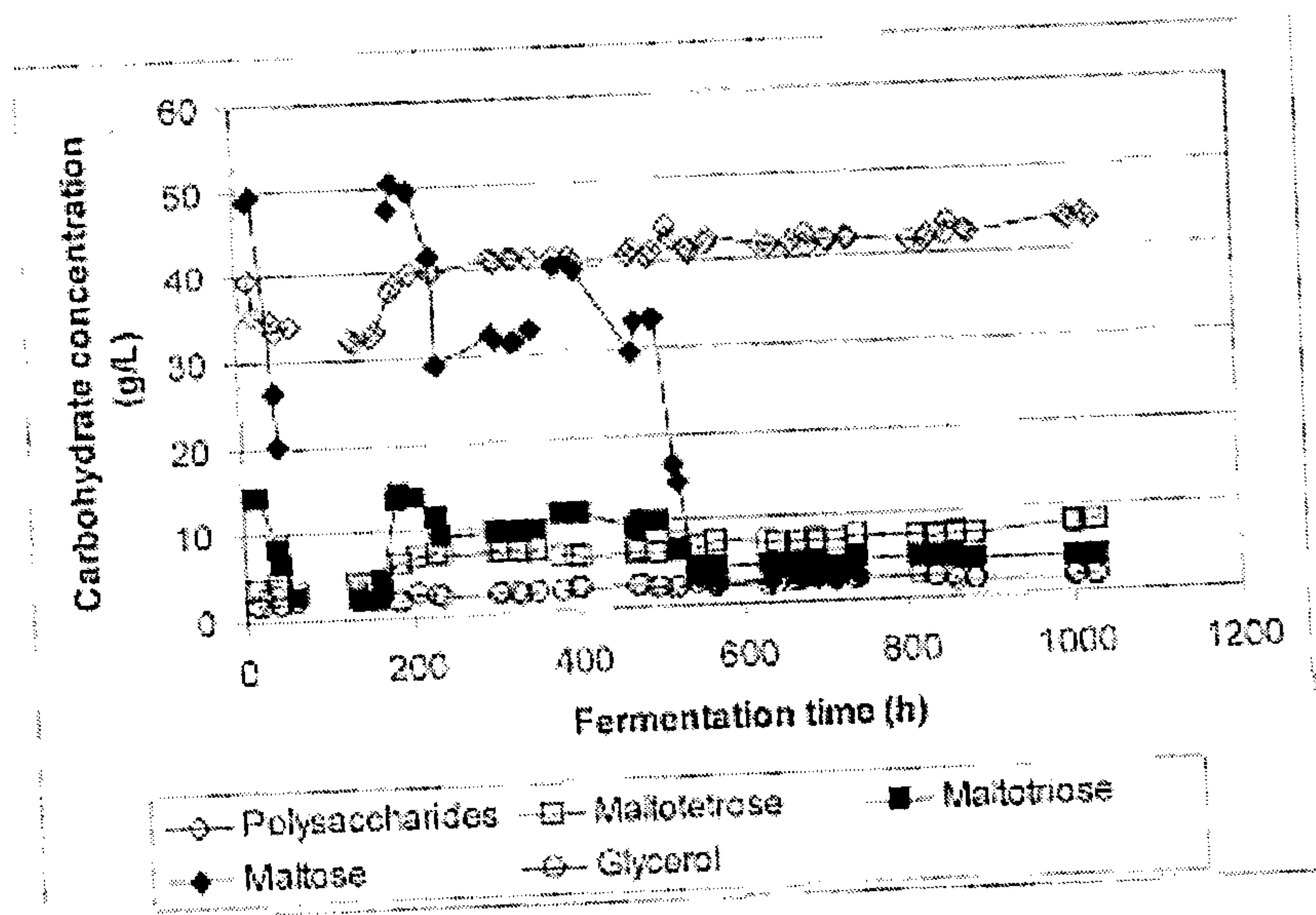
FIGURE 6.62 CARBOHYDRATES PROFILE OF CARRAGEENAN IMMOBILIZED YEAST CONTINUOUS FERMENTATION VERSUS FERMENTATION TIME.
