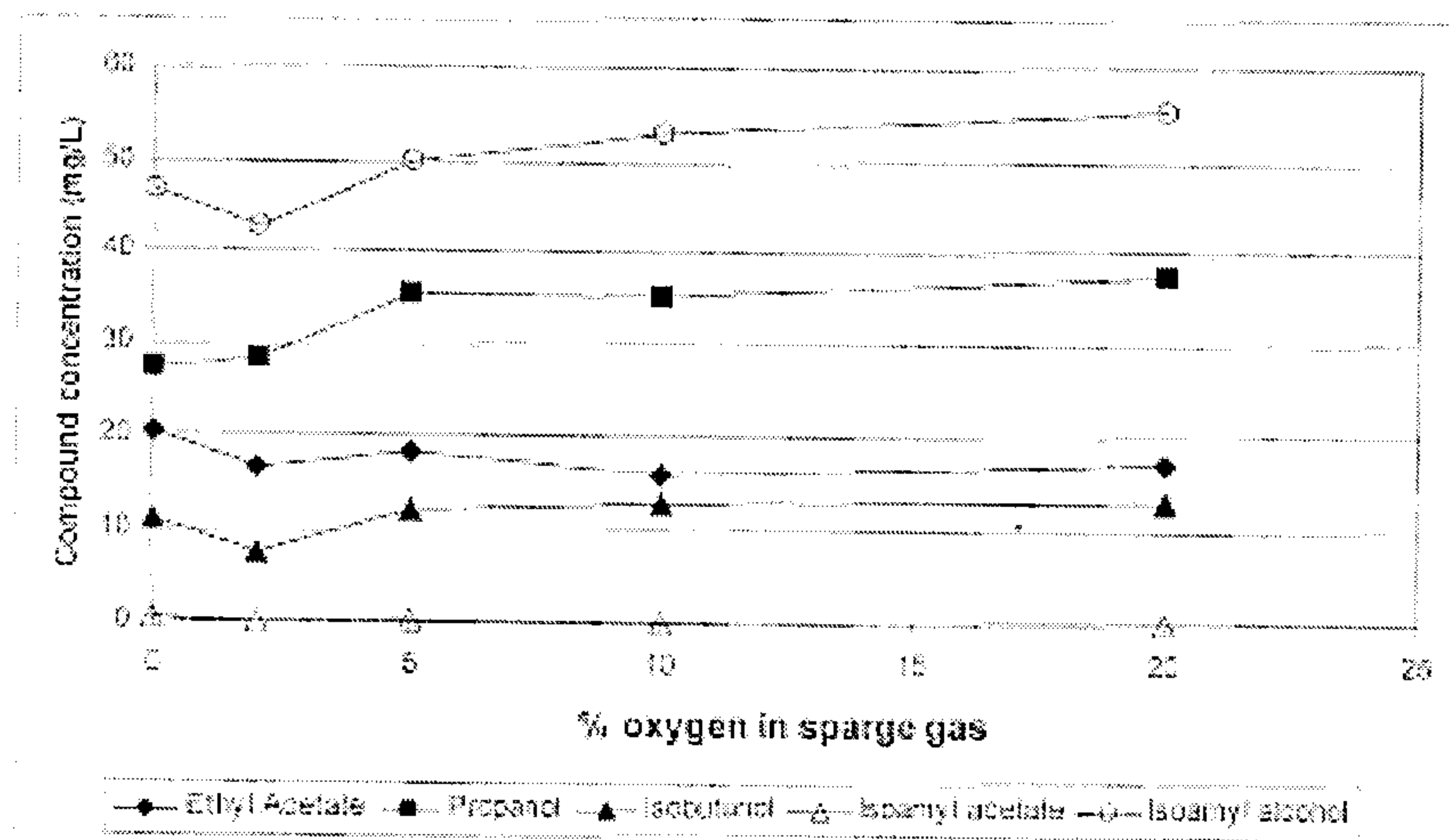
FIGURE 6.36 ESTERS AND FUSOL ALCOHOLS CONCENTRATION VERSUS PERCENT OXYGEN IN THE SPARGE GAS. THE FERMENTATIONS WERE CARRIED OUT IN THE 50-L GAS-LIFT SYSTEM LOADED WITH 40% (V/V) CARRAGEENAN GEL BEADS. THE TOTAL SPARGE RATE WAS KEPT CONSTANT AT 6.4 SCFH. THE RESIDENCE TIME WAS 24 HOURS.
