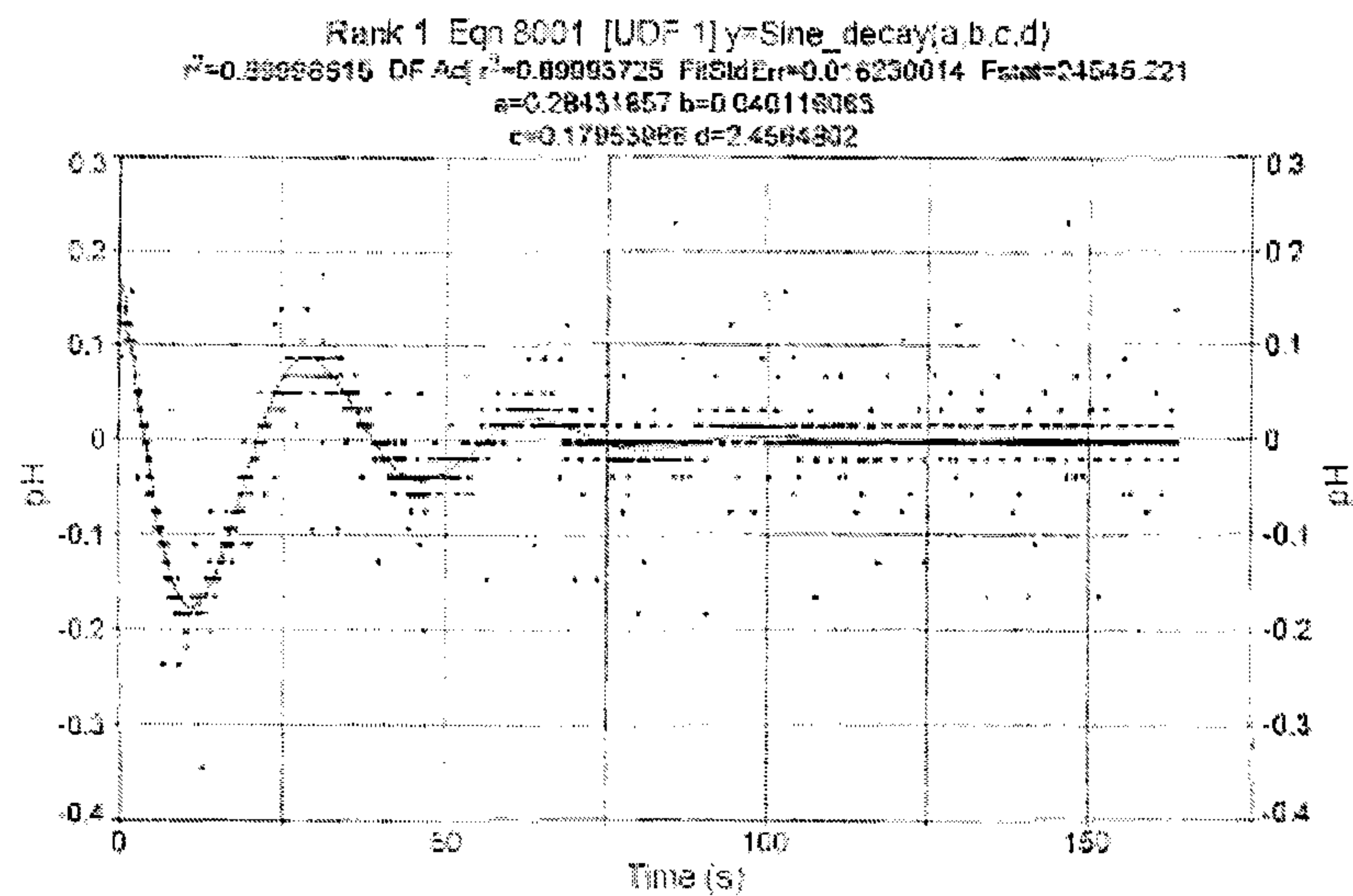
FIGURE 6.46 PH PROBE RESPONSE DATA WITHIN A 50 L GAS-LIFT DRAFT TUBE BIOREACTOR. AN ACID PULSE WAS INJECTED INTO A FERMENTATION MEDIUM CONTAINING THE HIGHLY FLOCCULENT YEAST, LCC298. THE SUPERFICIAL GAS VELOCITY WAS SET AT 1.94 MM/S. THE ORIGINAL DATA WAS FITTED TO A DECAYING SINUSOIDAL CURVE. THE COEFFICIENT OF CORRELATION WAS 0.99.
