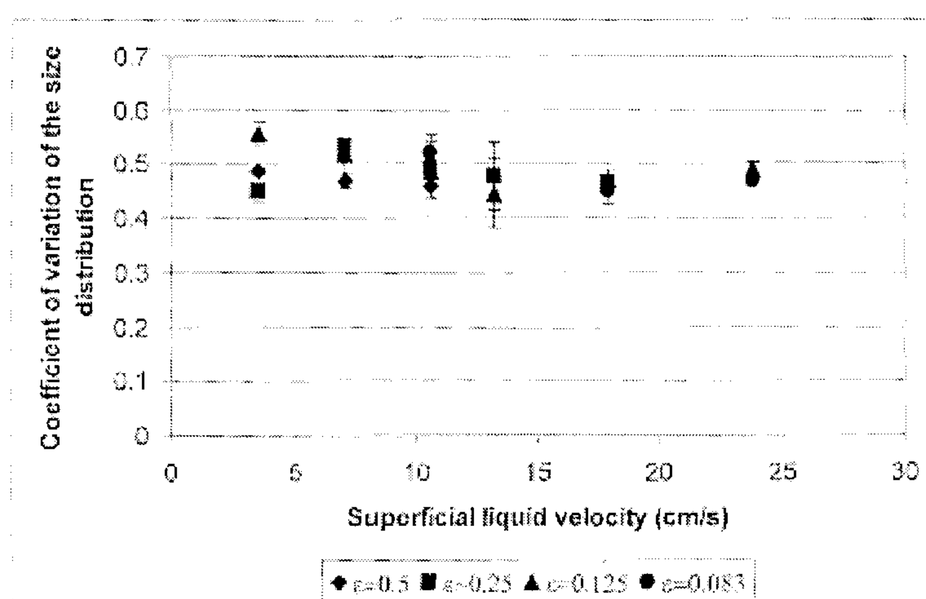
FIGURE 6.17. SUPERFICIAL LIQUID VELOCITY (CM/S) VERSUS COEFFICIENT OF VARIATION OF THE BEAD DIAMETER (%). FOUR POLYMER FRACTIONS ( \phi OF 0.5, 0.25, 0.125 AND 0.083) WERE EVALUATED. THE NUMBER OF STATIC MIXER ELEMENTS ( N_s ) WAS KEPT CONSTANT AT 48 AND THE STATIC MIXER DIAMETER ( D_s ) WAS SET AT 12.7 MM.
