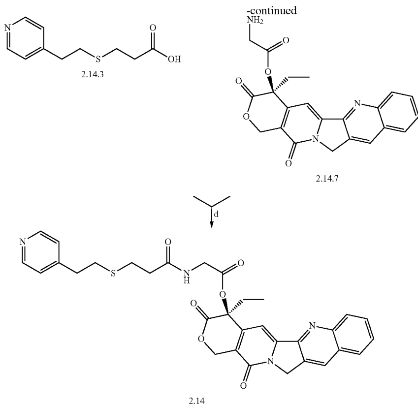
Scheme 1: Reagents and conditions:
