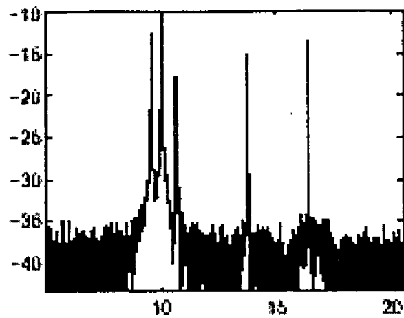
Figure 20: Upstream Channel Spectrum
