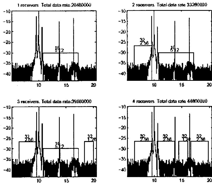
Figure 21: Allocation of 1-4 upstream channels (Note that the heights of the squares do NOT represent the allocated channel spectral density)
