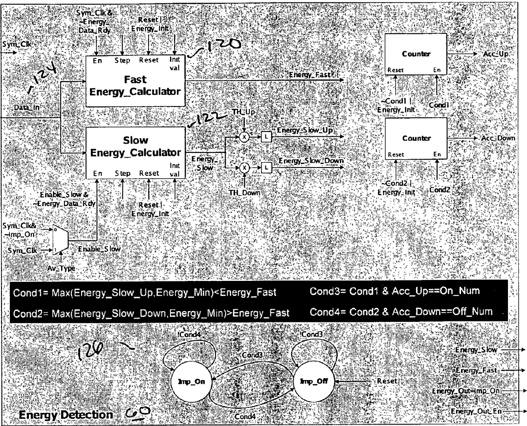
Figure 8: Energy detection method (time domain analyzer, low-level analysis) block diagram
