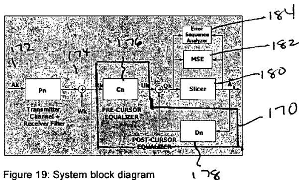
Figure 19: System block diagram
