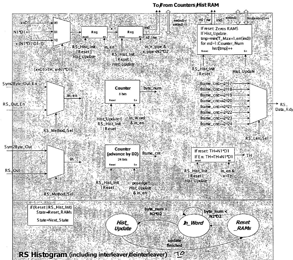
Figure 15: RS histogram block diagram & state machine (with interleaver/deinterleaver)
