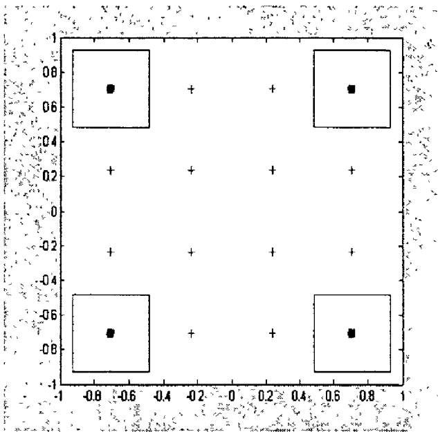
Figure 10:Soft decision method (time domain analyzer, low-level analysis)
