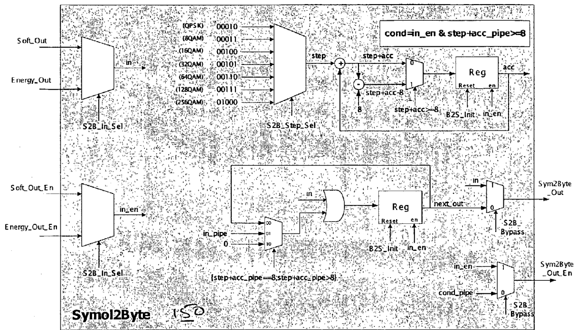
Figure 18: Symbol2Byte module block diagram
