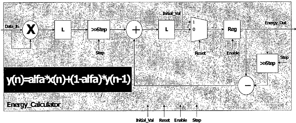
Figure 7: Energy calculator block diagram
