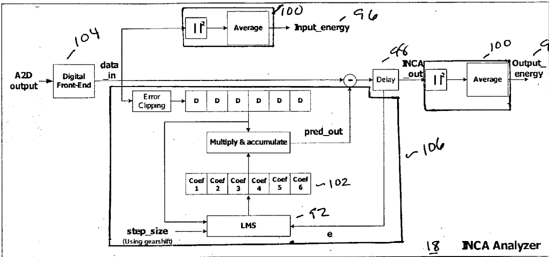
Figure 6: INCA Analyzer block diagram
