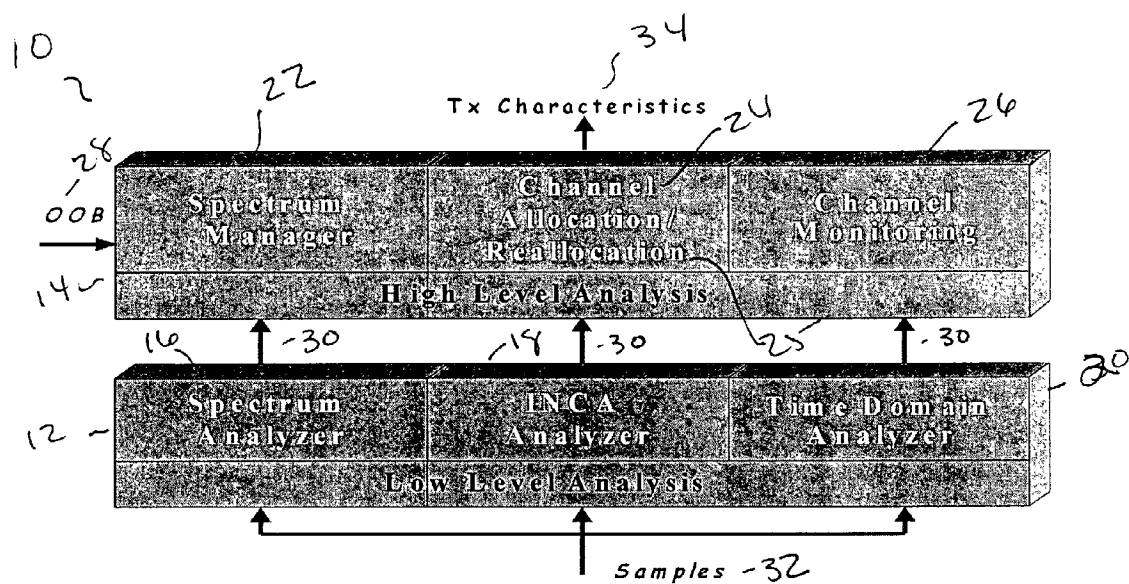
Figure 1: DUCA block diagram
