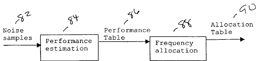
Figure 5: A system for allocating QAM signals
