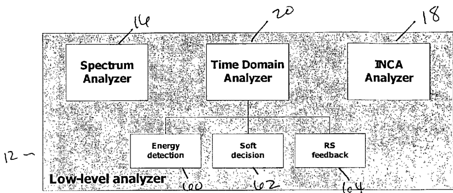
Figure 3: Low-level analyzer block diagram
