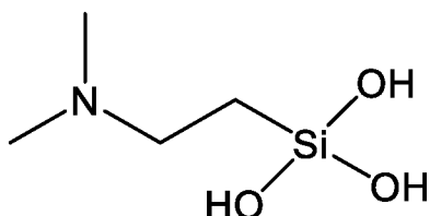
-1-(2-Dimethaminoethyl)silanetriol
