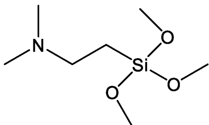
-1-(2-Dimethaminoethyl)silanetriol
