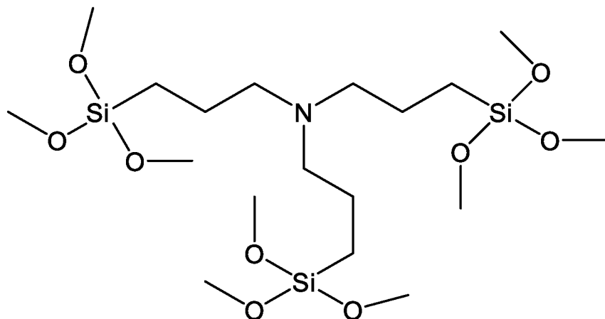
- 3-(Trimethoxysilyl)-N,N-bis[3-(trimethoxysilyl)propyl]-1-propanamin
