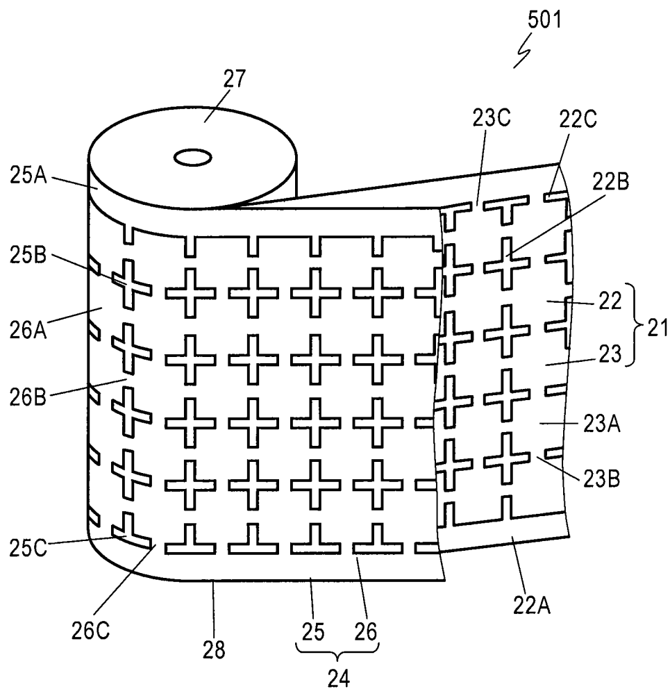
Fig. 9 Prior Art
