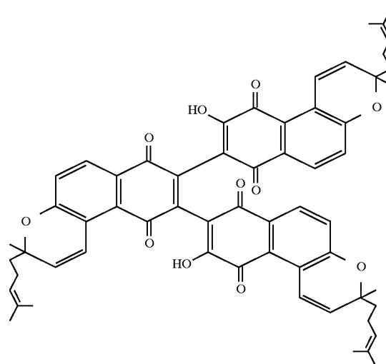
COMPOUND 1 (conocurvone)
