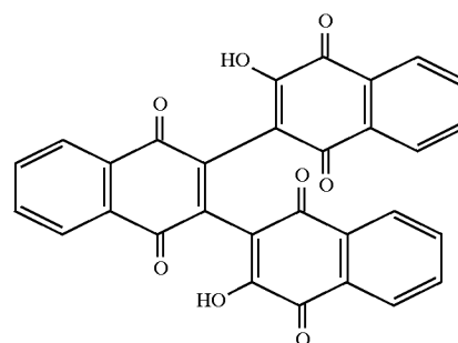
COMPOUND 9
