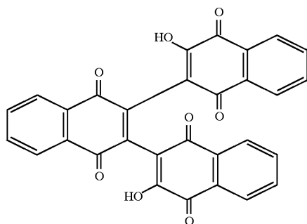
COMPOUND 9
