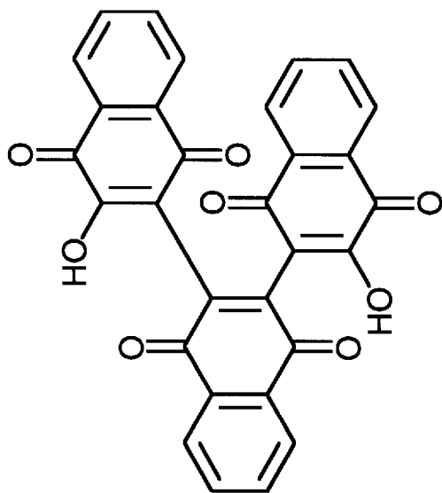
COMPOUND 9
