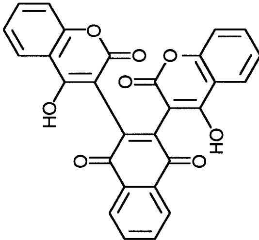
COMPOUND 10
