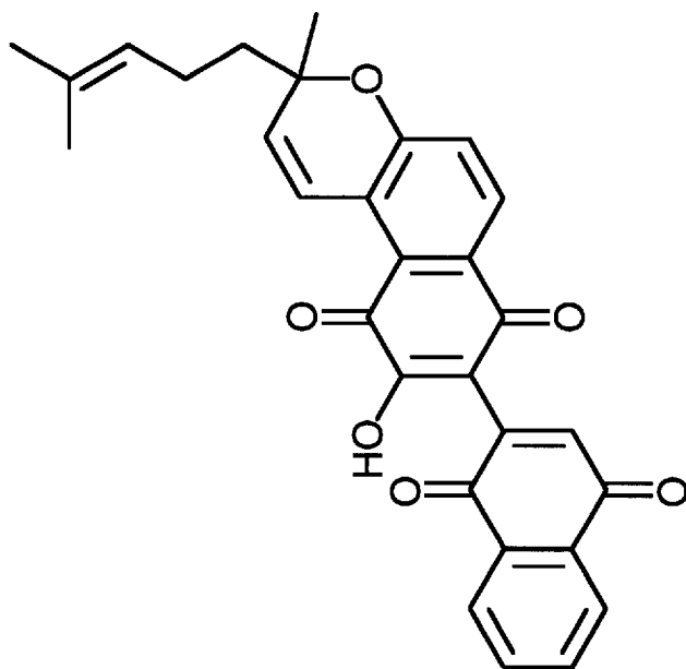
COMPOUND 5
