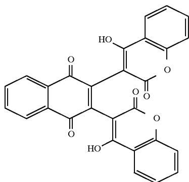
COMPOUND 10
