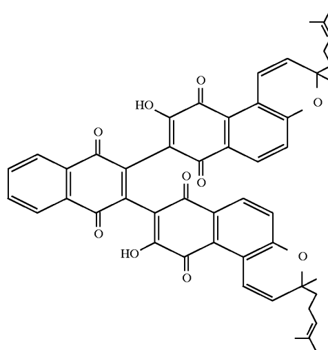
COMPOUND 4
