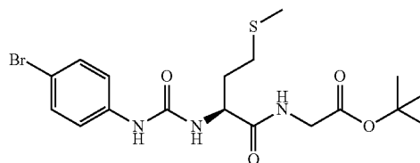
tert-butyl{{[(2S)-2-{{[(4-bromophenyl]carbamoyl}amino)-4-(methylsulfonyl)butanoyl]amino}acetate
