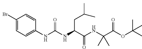
tert-butyl 2-{{[(2S)-2-{{[(4-bromophenyl]carbamoyl}amino)-4-methylpentanoyl]amino}-2-methylpropanoate
