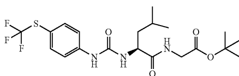
tert-butyl {{[(2S)-4-methyl-2-({[4-(trifluoromethyl)sulfanyl]phenyl]carbamoyl}amino)pentanoyl]amino}acetate
