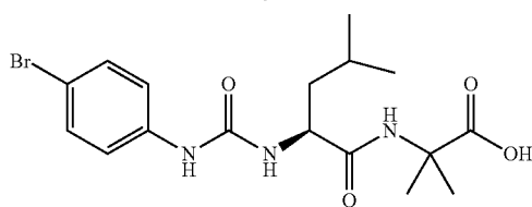
2-{{[(2S)-2-{{[(4-bromophenyl]carbamoyl}amino)-4-methylpentanoyl]amino}-2-methylpropanoic acid
