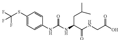
{{[(2S)-4-methyl-2-({[4-(trifluoromethyl)sulfanyl]phenyl]carbamoyl}amino)pentanoyl]amino}acetic acid
