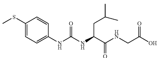
{{[(2S)-4-methyl-2-({[4-(methylsulfonyl)phenyl]carbamoyl}amino)pentanoyl]amino}acetic acid
