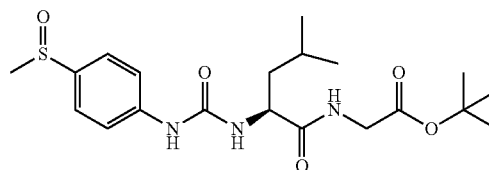
tert-butyl{{[(2S)-4-methyl-2-({[4-(methylsulfonyl)phenyl]carbamoyl}amino)pentanoyl]amino}acetate
