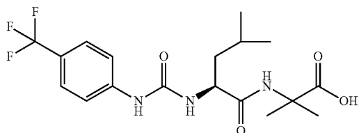
2-methyl-2-{{[(2S)-4-methyl-2-({[4-(trifluoromethyl)phenyl]carbamoyl}amino)pentanoyl]amino}propanoic acid
