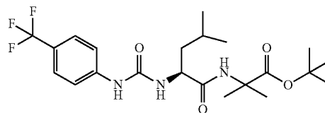
tert-butyl 2-methyl-2-{{[(2S)-4-methyl-2-({[4-(trifluoromethyl)phenyl]carbamoyl}amino)pentanoyl]amino}propanoate
