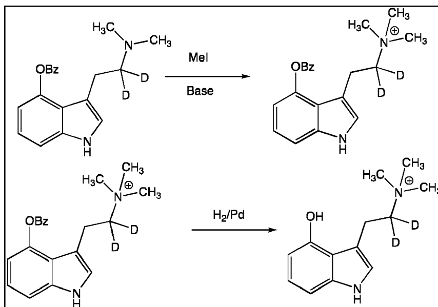
Scheme 2. Synthesis of Aer- \alpha,\alpha ,-d 2
