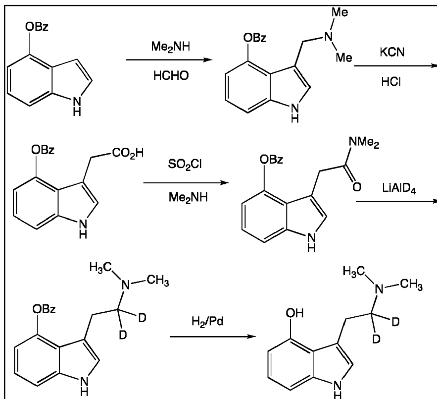
Scheme 1. Synthesis of PI- \alpha,\alpha -d 2 .
