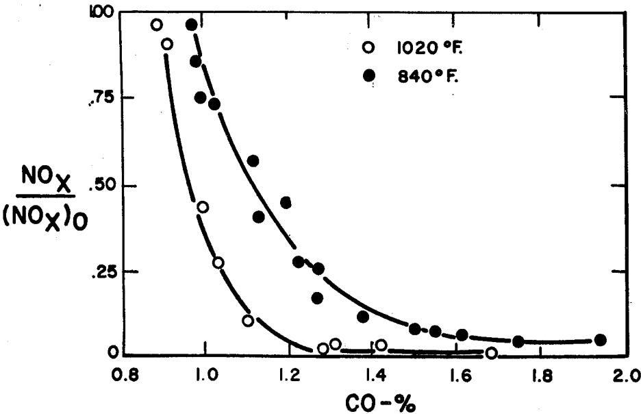
ACTIVITY FOR COPPER-PLATED STAINLESS STEEL 11.2 SCFM/LB.
