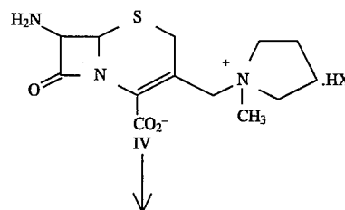
Reaction Scheme 2
