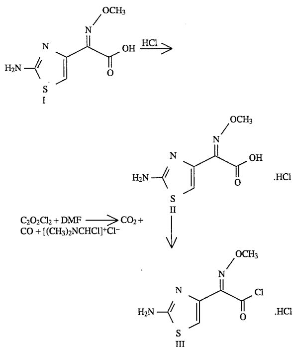
Reaction Scheme 1
