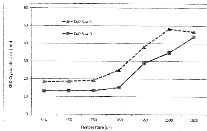
Figure 1. Crystallite sizes of Two Different Copper Oxide particles (CuO Raw C and CuO Raw D), both untrated, and heat treated at selected values from 450 °F to 1625 °F.
